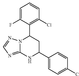
7-(2-chloro-6-fluorophenyl)-5-(4-chlorophenyl)-4,5,6,7-tetrahydro[1,2,4]triazolo[1,5-a]pyrimidine
