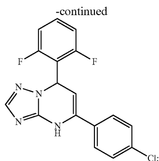
5-(4-chlorophenyl)-7-(2,6-difluorophenyl)-4,7-dihydro[1,2,4]triazole[1,5-a]pyrimidine
