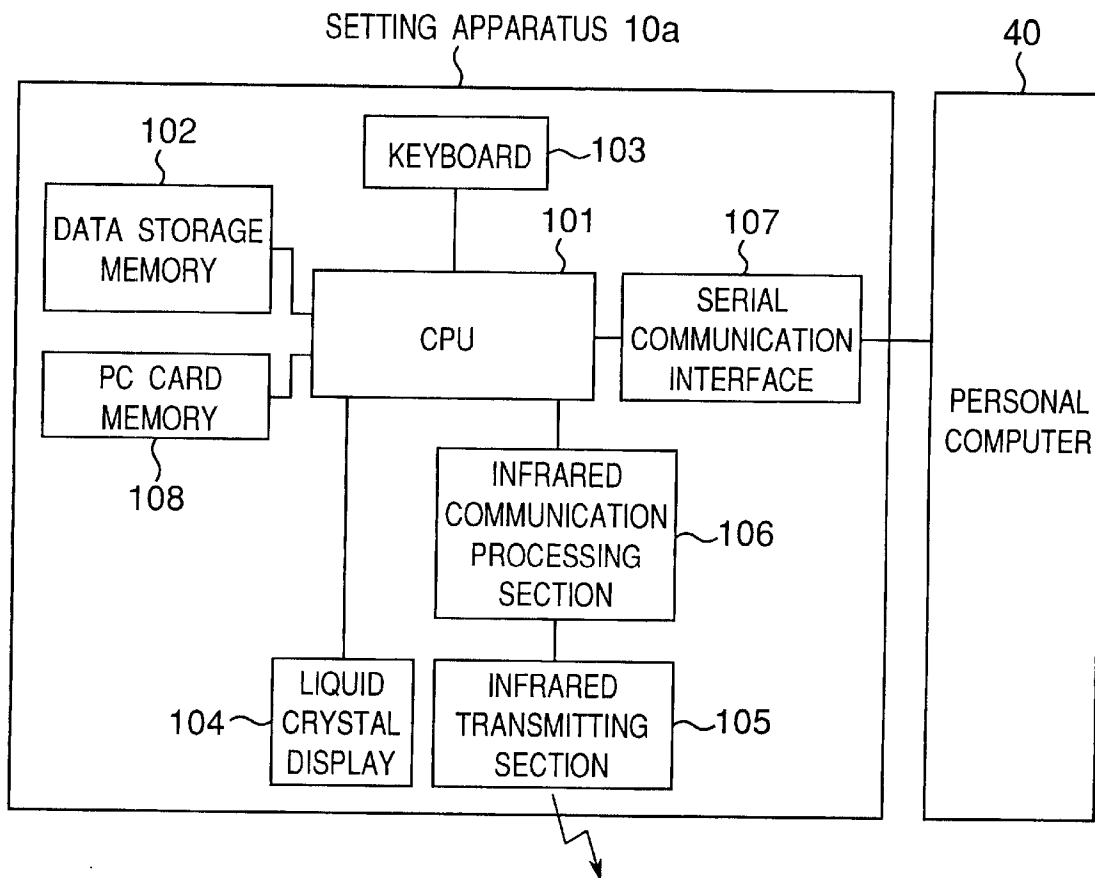
Fig.6 MODIFIED PREFERRED EMBODIMENT
