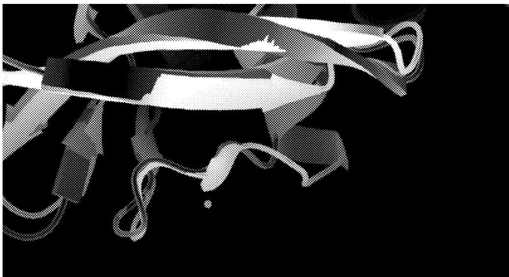
Figure 3 Close-up 3 residue deletion in PehPro1 structure.
