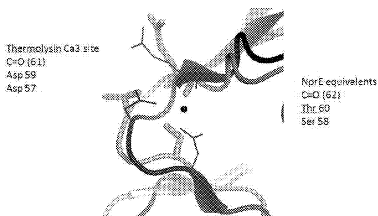
Figure 14 Comparison of NprE variant with Thermolysin at the region of Ca3 site, showing Calcium ion bound to Thermolysin as a sphere, while NprE lacks calcium ion.
