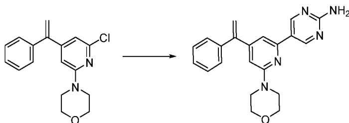
Compound 126
