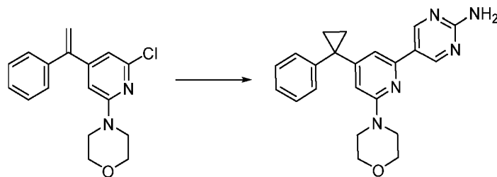
Compound 127
