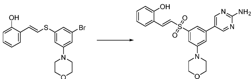
Compound 113
