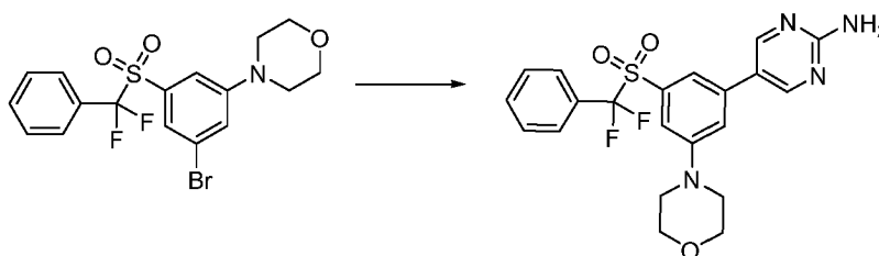
Compound 87
