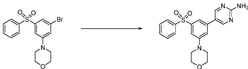
Compound 1
