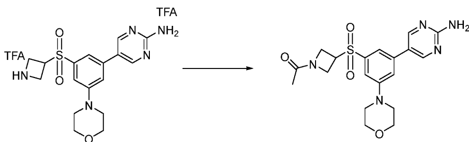
Compound 68
