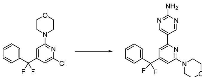
Compound 123
