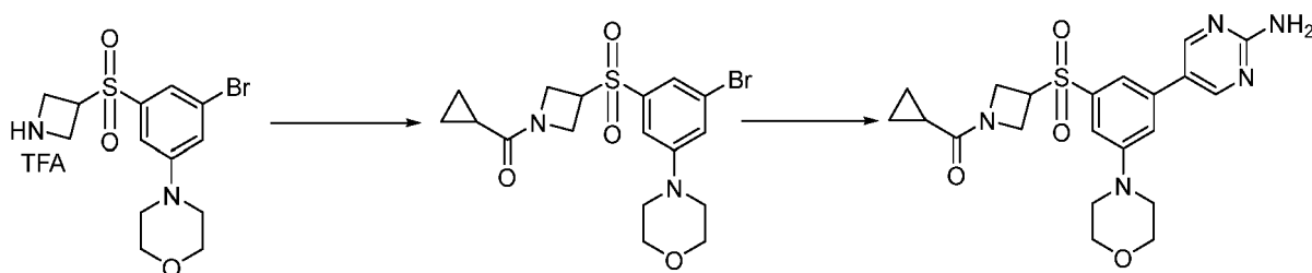
Compound 77
