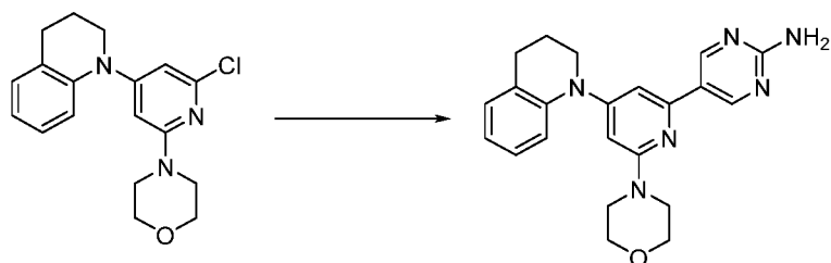
Compound 140
