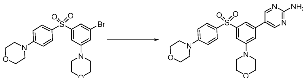
Compound 36
