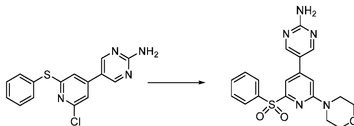
Compound 118
