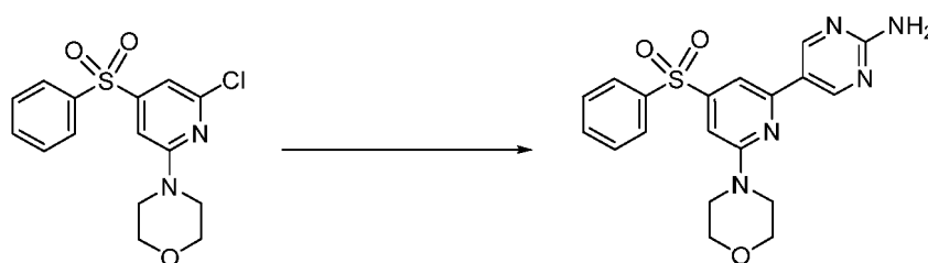
Compound 115
