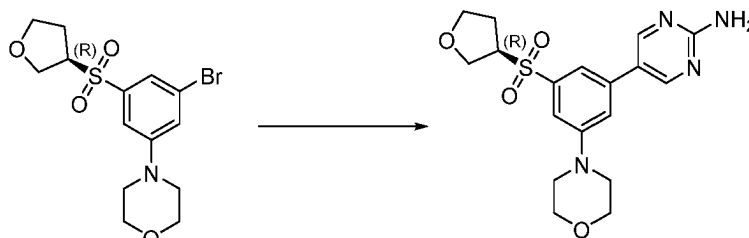
Compound 52
