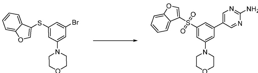
Compound 109
