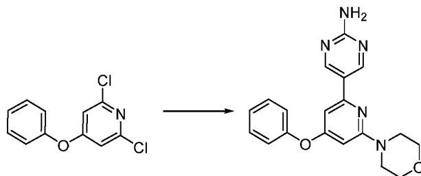
Compound 120
