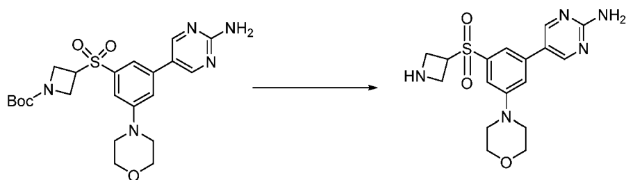
Compound 61
