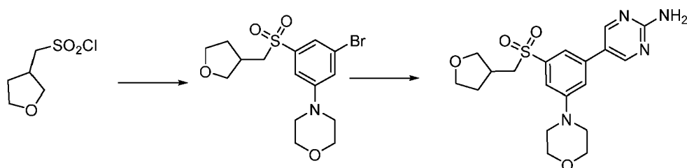
Compound 38
