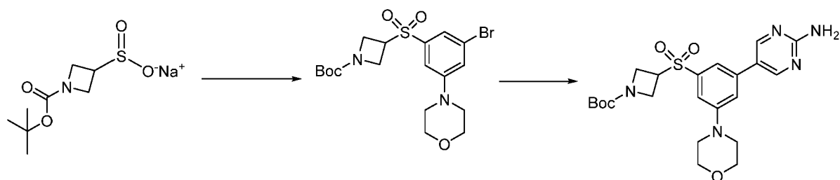
Compound 54
