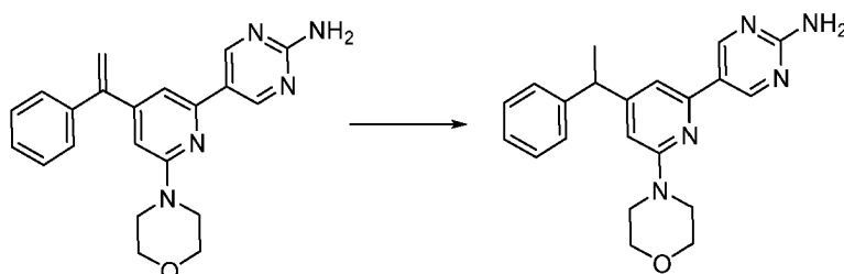
Compound 125
