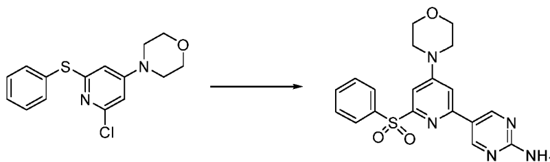
Compound 117
