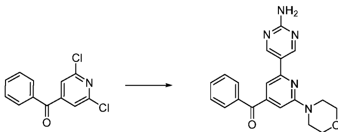
Compound 122
