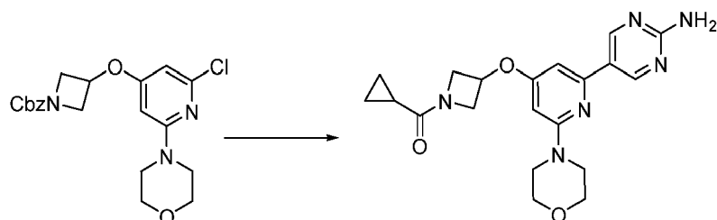
Compound 129
