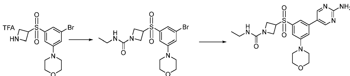
Compound 93
