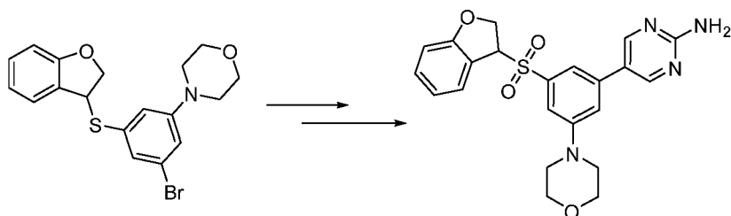
Compound 119
