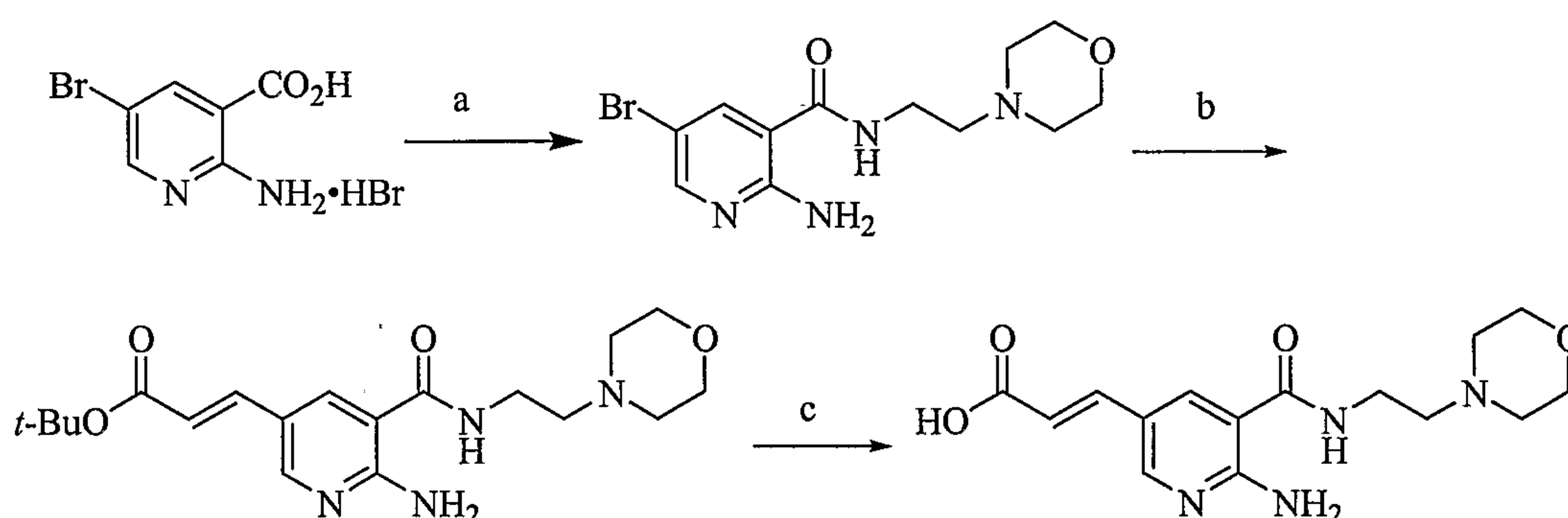
Scheme XX
