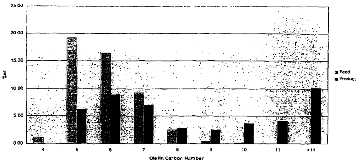
Olefin Shift from Fractionation Data
