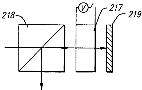
TRANSMITTED
