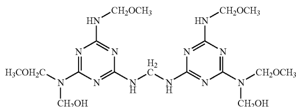
Structure of Cymel® 385 dimer
