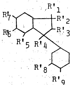
cyclohexyl hydrindan
