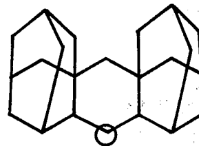
Cis-type
