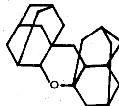
Cis-type
