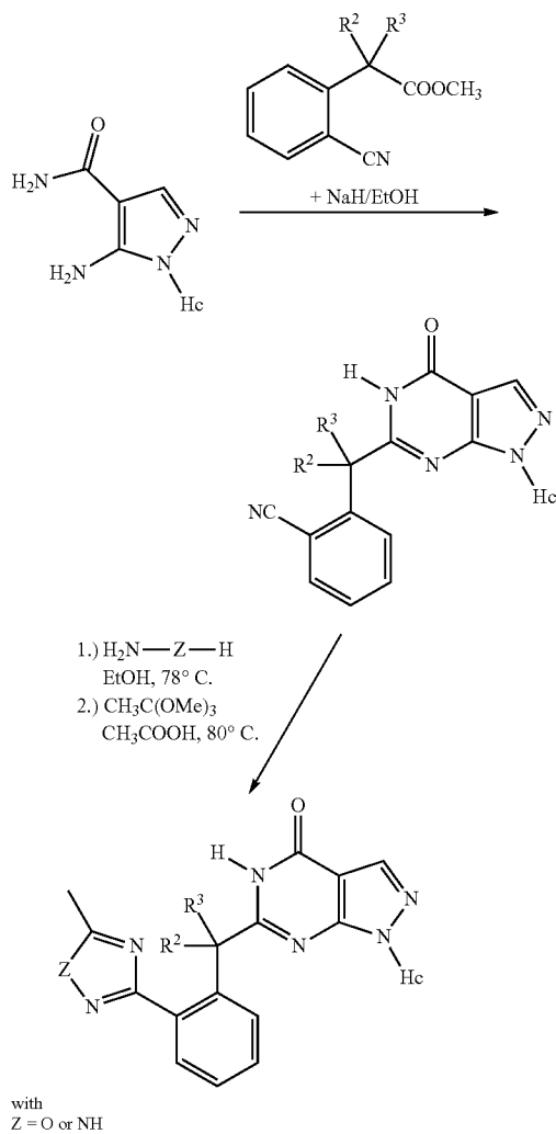
Scheme 7
