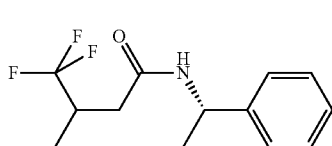
Diastereoisomer A
