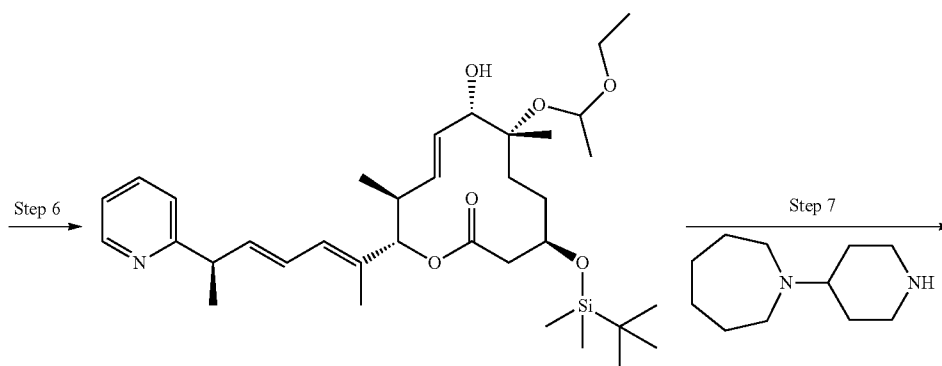
Scheme III
