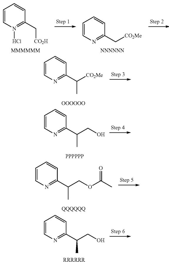
Scheme V
