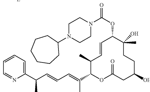
Compound 1
