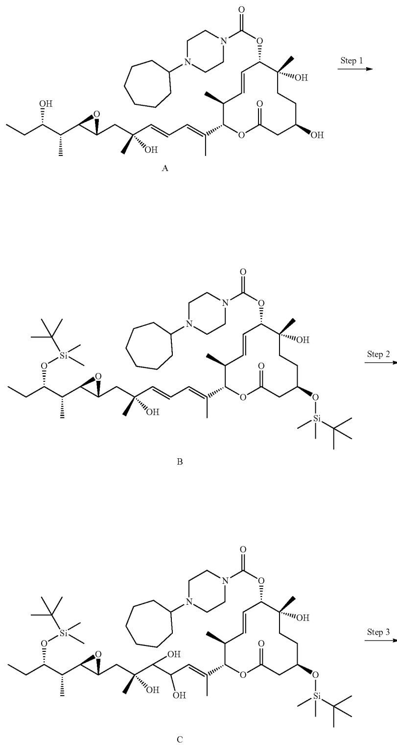
Scheme I
