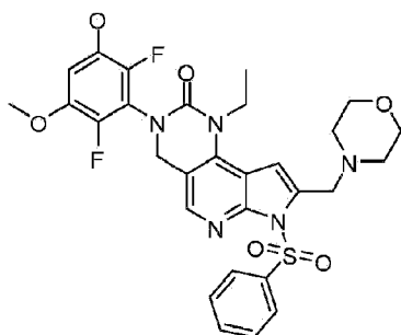
Compound 8;
