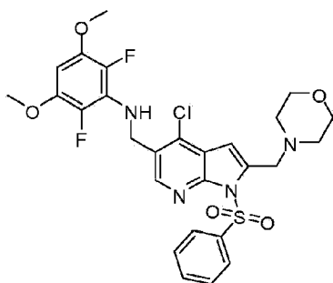
Compound 6;
