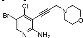
Compound 9.
