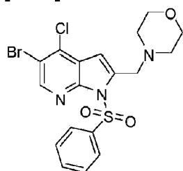
Compound 11.
