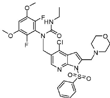
Compound 7;
