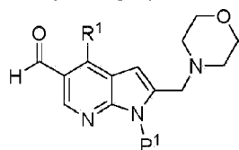
Compound F4
