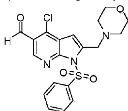
Compound 4;
