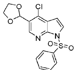
Compound 2
