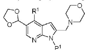
Compound F3
