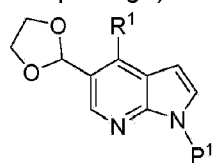
Compound F2
