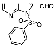
Compound 2a;
