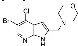
Compound 10
