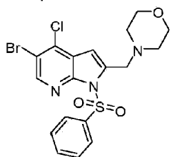
Compound 11
