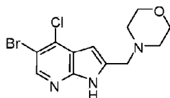
Compound 10
