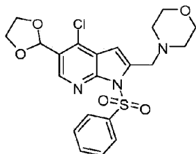
Compound 3;
