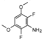
Compound 5
