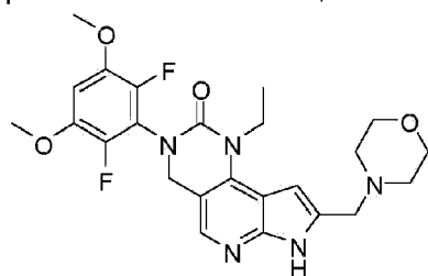
Compound 1,
