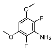
Compound F5
