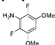
Compound 5
