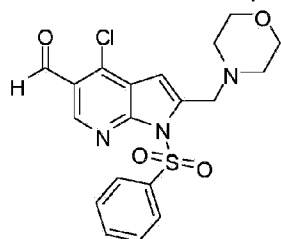
Compound 4
