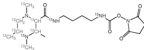
CN(C)C(=O)NCCCCNC(=O)Oc1cc(=O)[nH]c1=O
