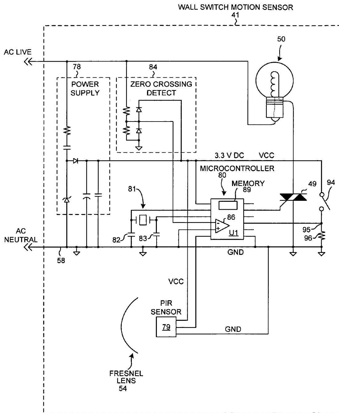
WALL SWITCH MOTION SENSOR CIRCUIT
