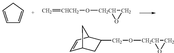
FIG. 1 was a scheme shown the process to prepare various cross-linked hybrid materials from norbornene compound with cross-linkable groups.
