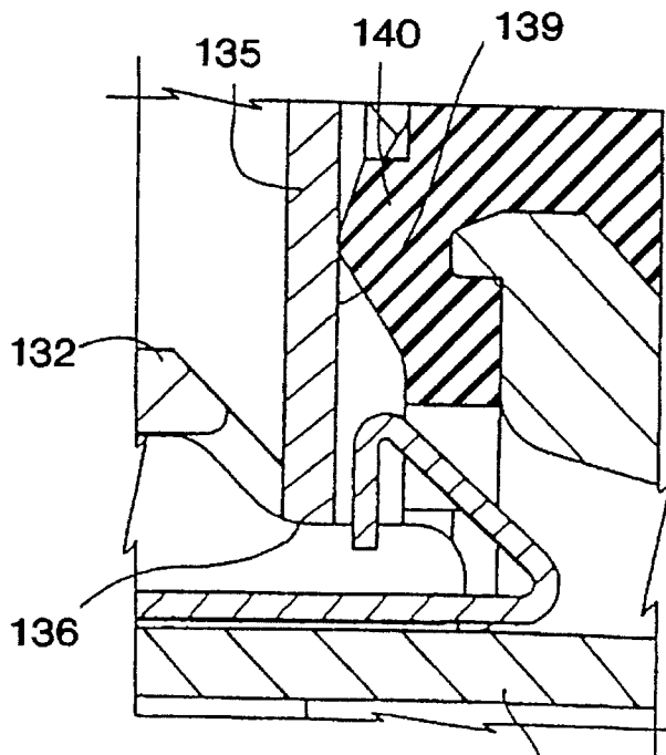
FIG. 9 PRIOR ART
