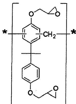
JER-157S65
