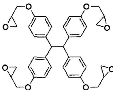
JER-10315
