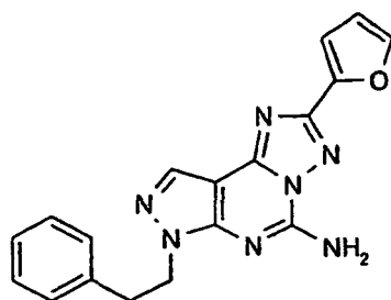
Sch-58261
