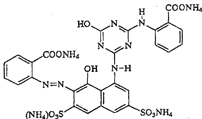
Compound A
