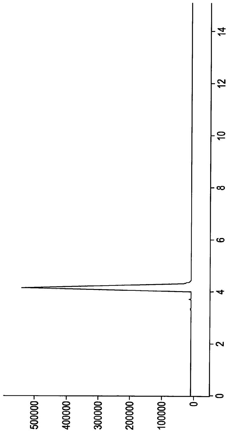
FIG. 3 1, 8-bis(cyclohexylamino) anthraquinone
