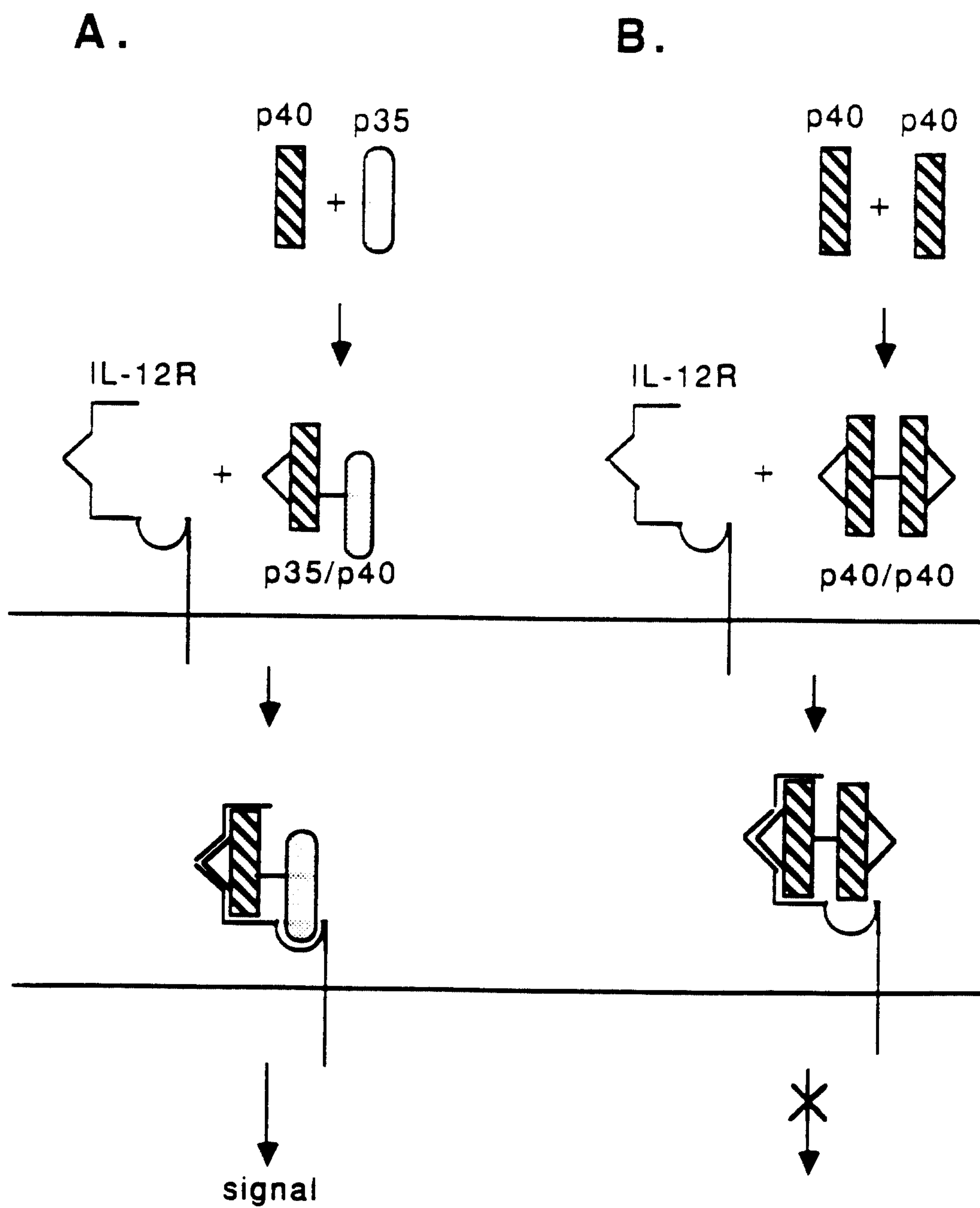
Model of IL-12 Binding and Signaling
