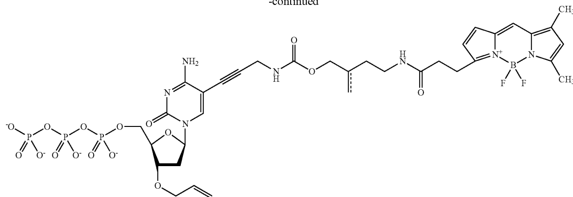
3'-O-allyl-dCTP-allyl-Bodipy-FL-510
