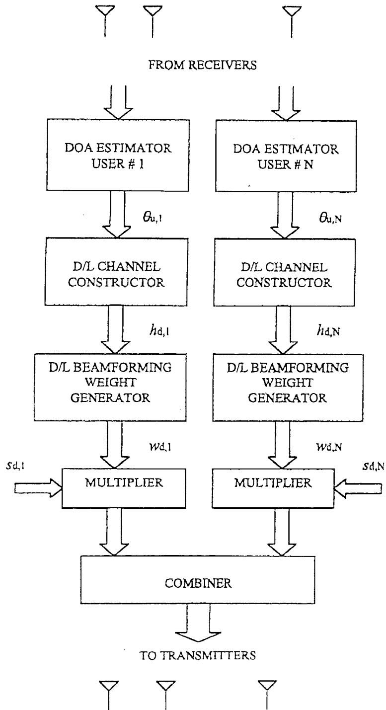
FIG.1 PRIOR ART
