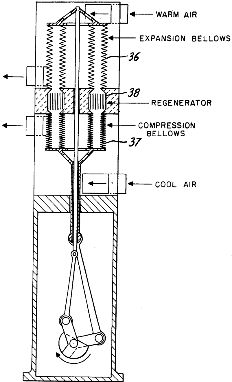
BELLOWS ISOTHERMAL HEAT ENGINE
