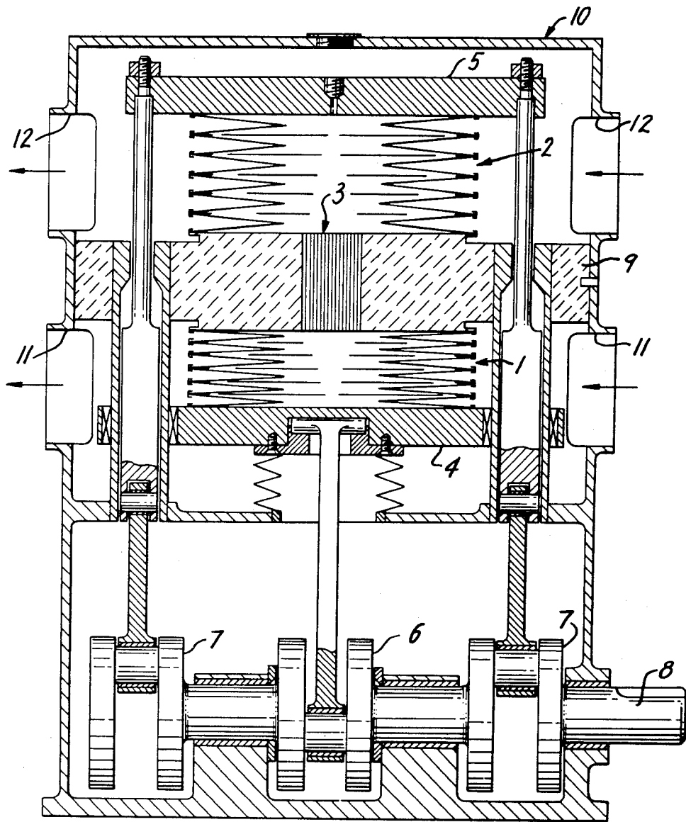
BELLOWS HEAT PUMP WITH CRANKSHAFT DRIVE
