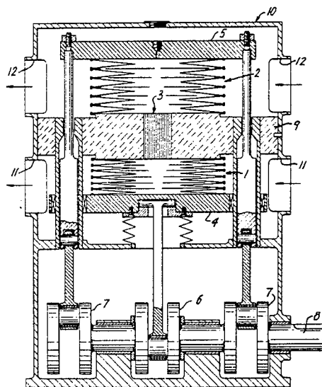
BELLOWS HEAT PUMP WITH CRANKSHAFT DRIVE
