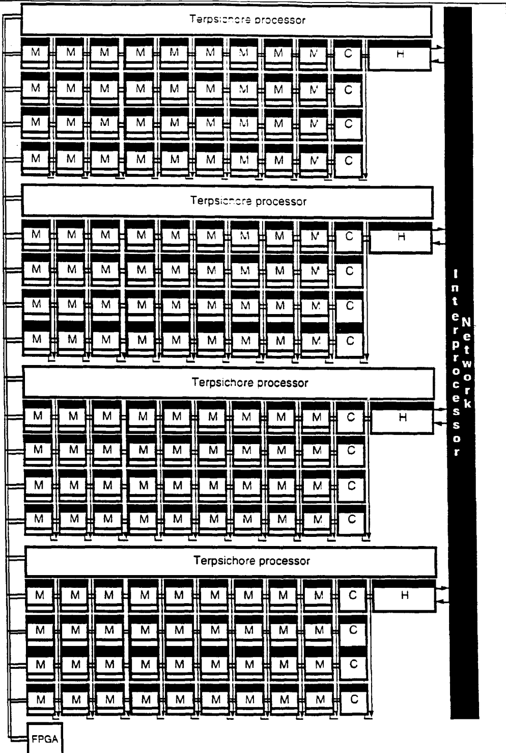
Maximum Terpsichore system application four minimally-configured processors per board
