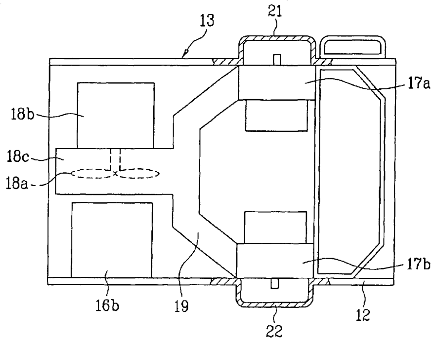
FIG. 3 Related Art
