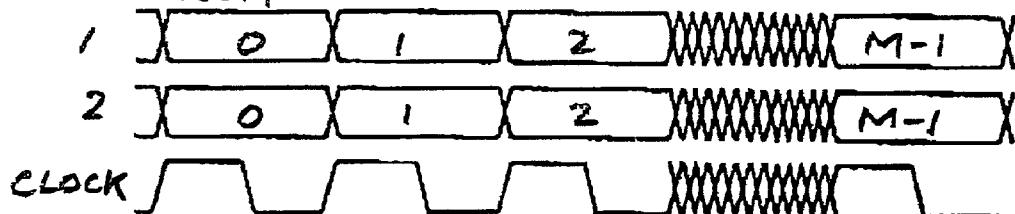
OUTPUT OF PIXEL DATA REARRANGEMENT CIRCUIT
