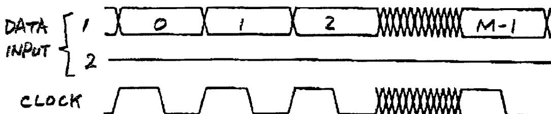
DATA FORMAT 1
