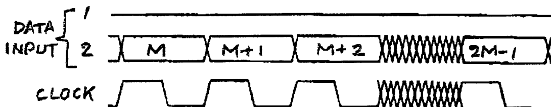
DATA FORMAT 2
