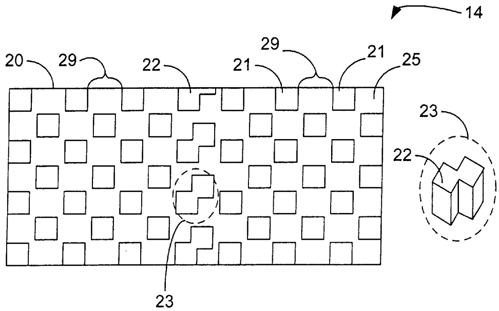
FIG. 2 (PRIOR ART)
