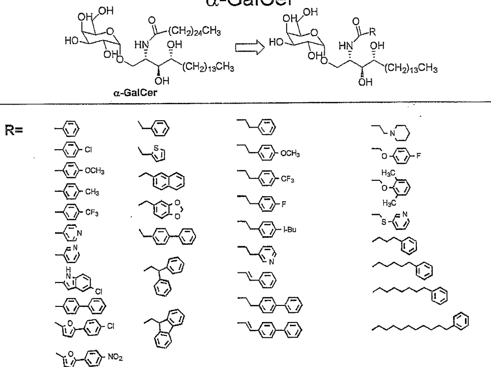
Scheme 1 Synthesis of fatty acid chain analogs of \alpha -GalCer
