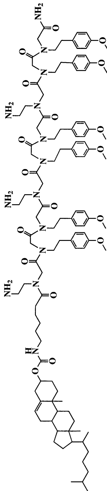
Chol-Ahx-(NaeNmpeNmpe) 3
