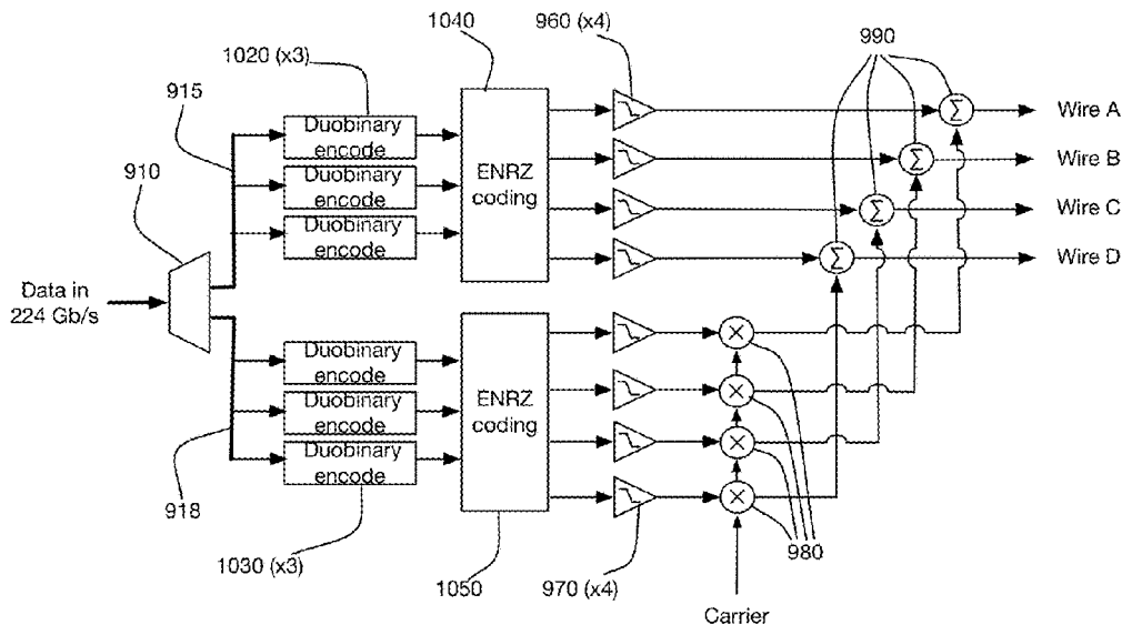
Alternative Transmitter
