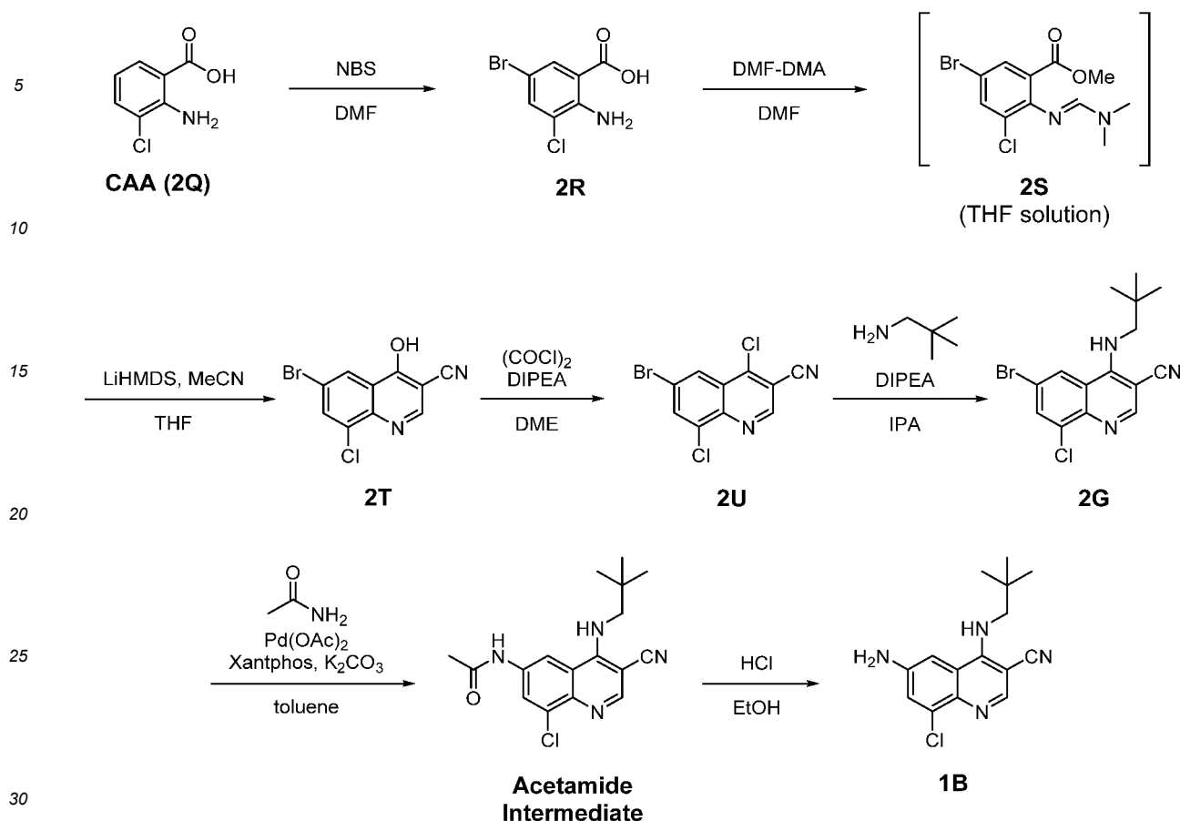
Scheme 7
