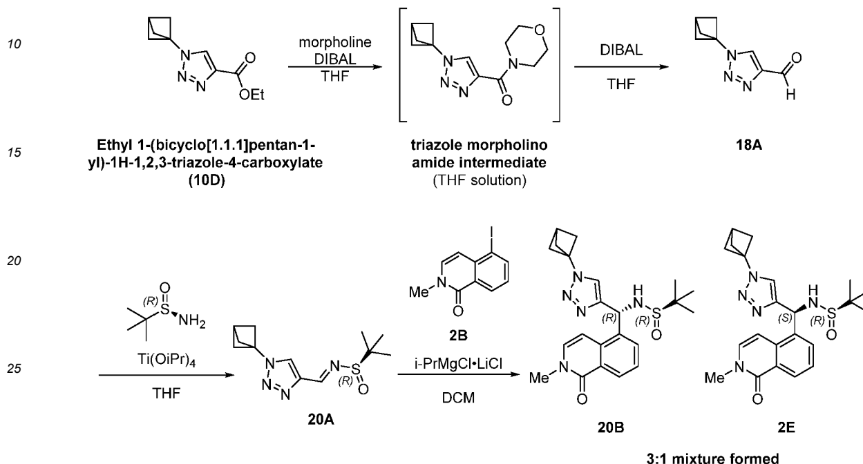
Scheme 21A
