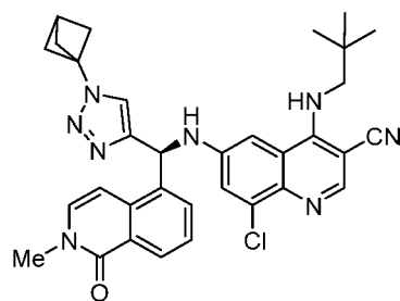
Compound 1
