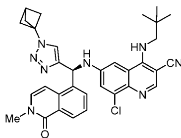
Compound 1
