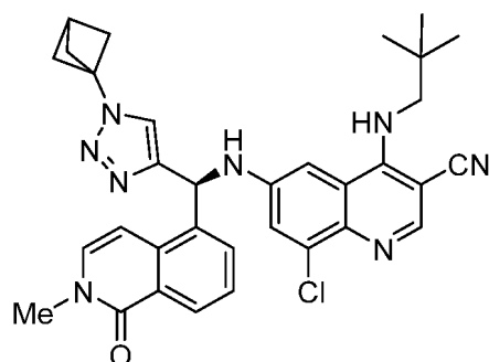
Compound 1
