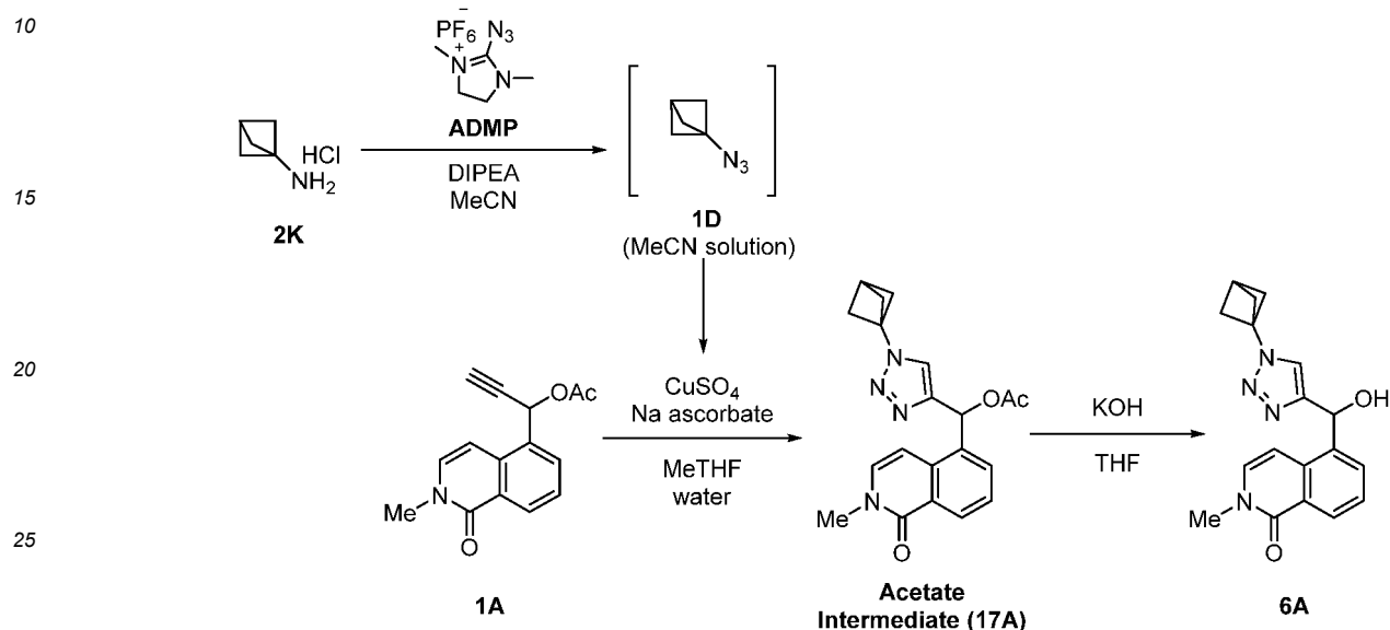
Scheme 18
