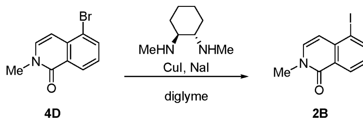
Scheme 16
