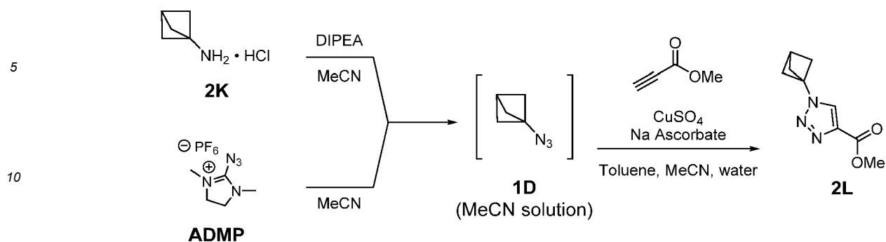
Scheme 12
