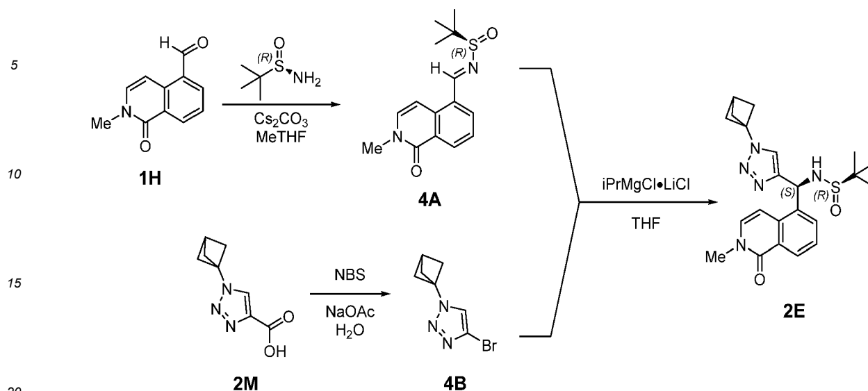
Scheme 9
