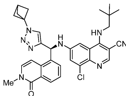
Compound 1
