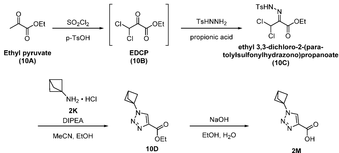
Scheme 11
