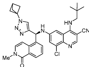
Compound 1
