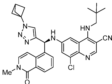
Compound 1
