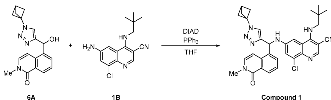
Scheme 24
