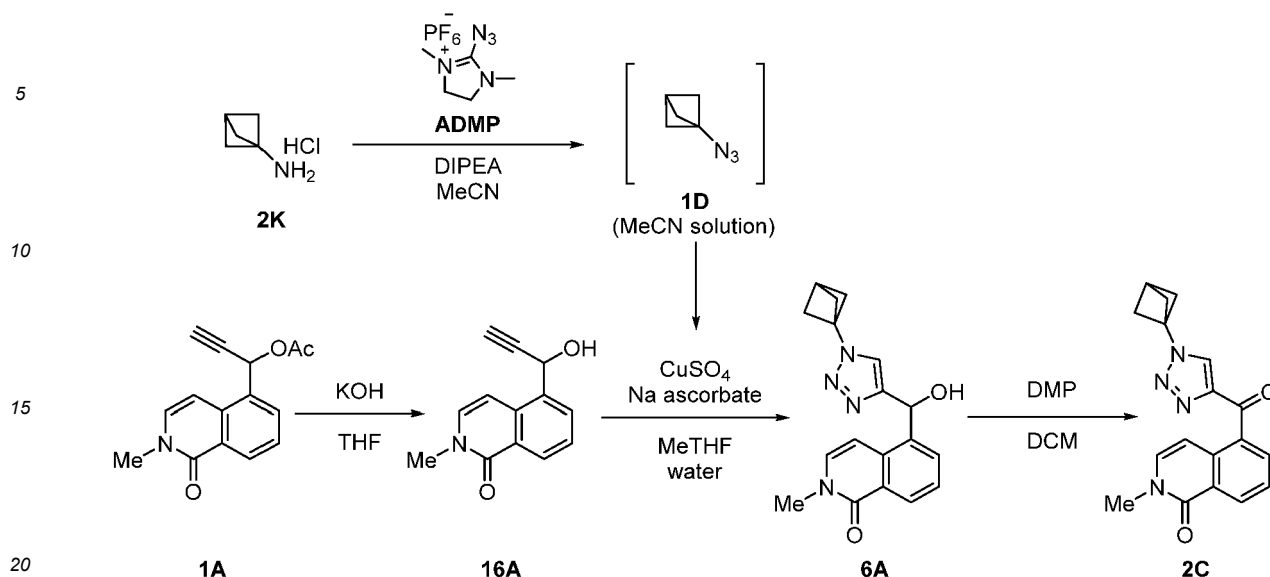
Scheme 17
