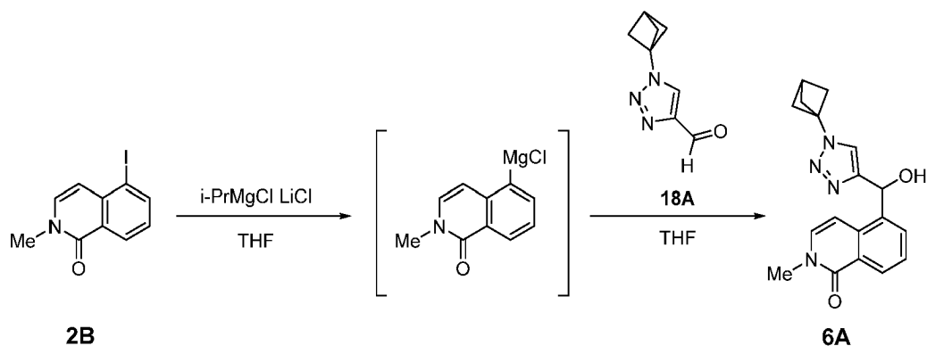
Scheme 19
