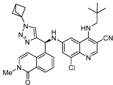
Compound 1
