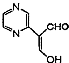
C-13
