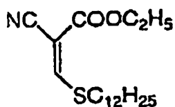
C-17
