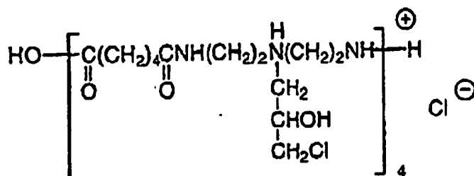
Compound H
