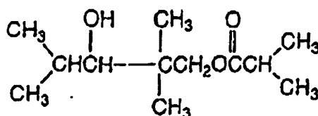
Compound F
