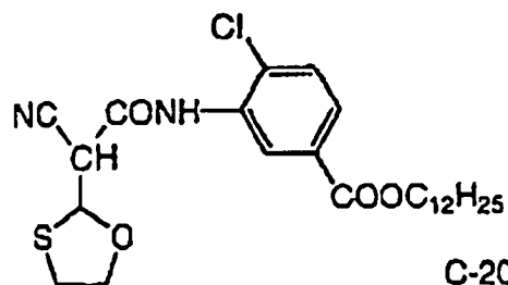
C-17
