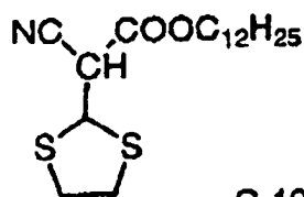
C-19
