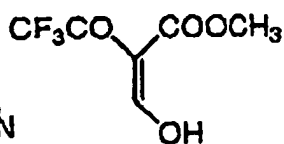
C-10
