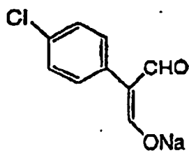
C-14
