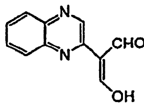
C-15
