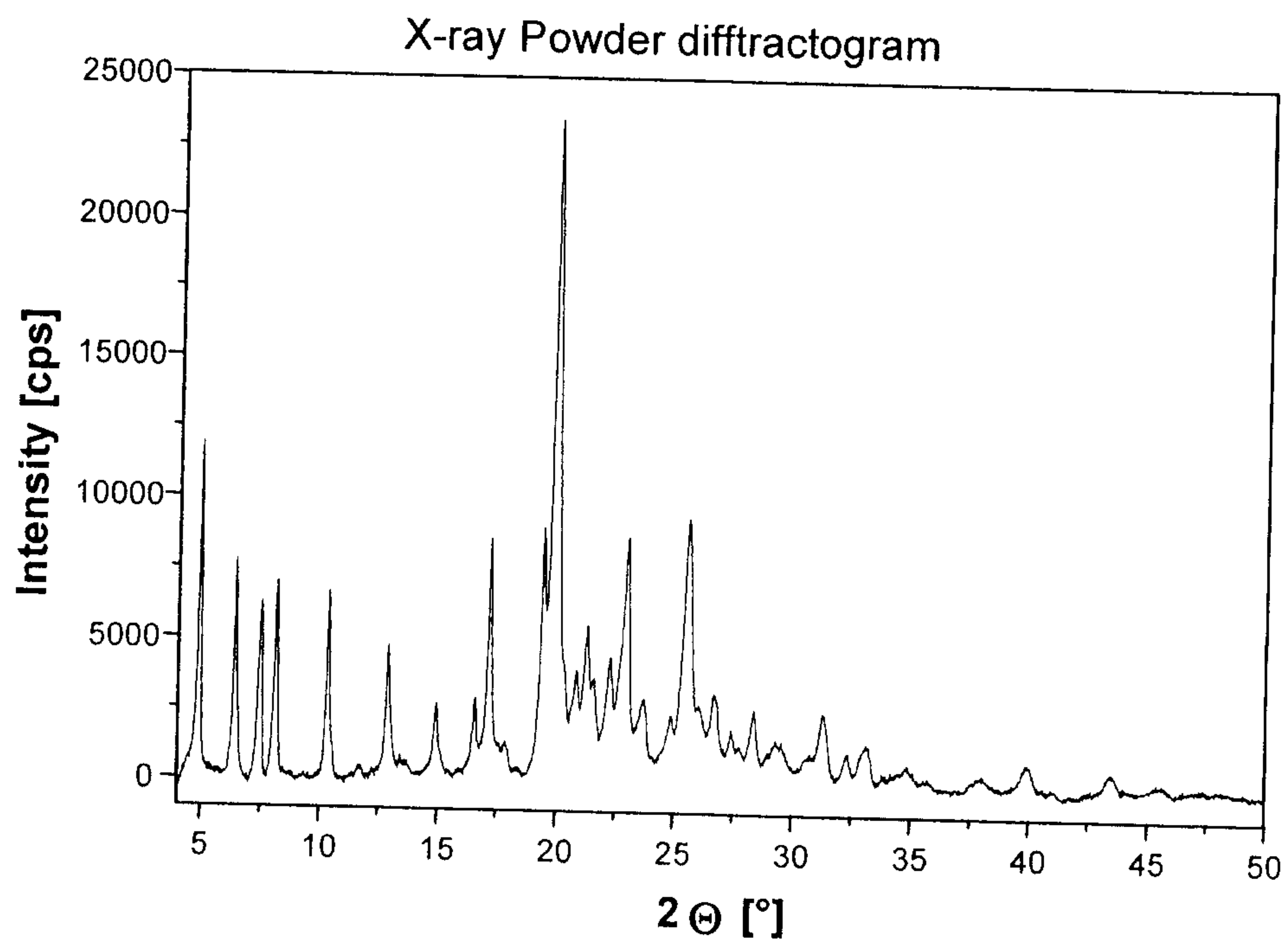
Figure 1: X-ray powder diffractogram of 4-[(3-chloro-4-fluorophenyl)amino]-6-[[4-(N,N-dimethylamino)-1-oxo-2-buten-1-yl]amino]-7-((S)-tetrahydrofuran-3-yloxy)-quinazoline dimaleate
