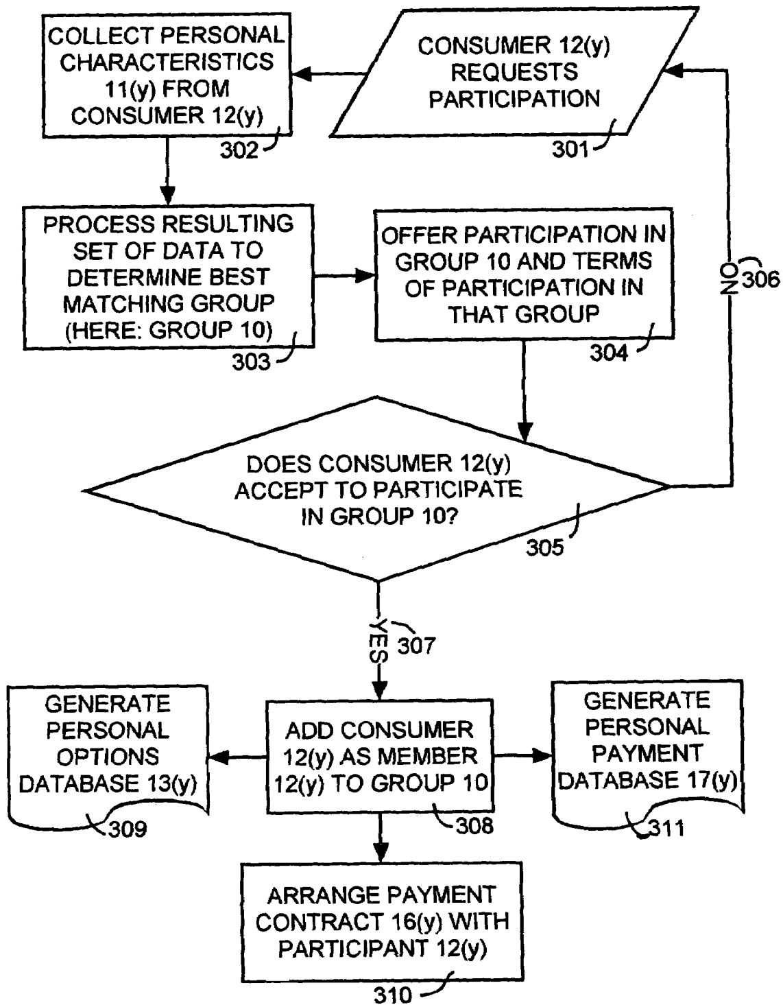
Fig.3: Group Forming
