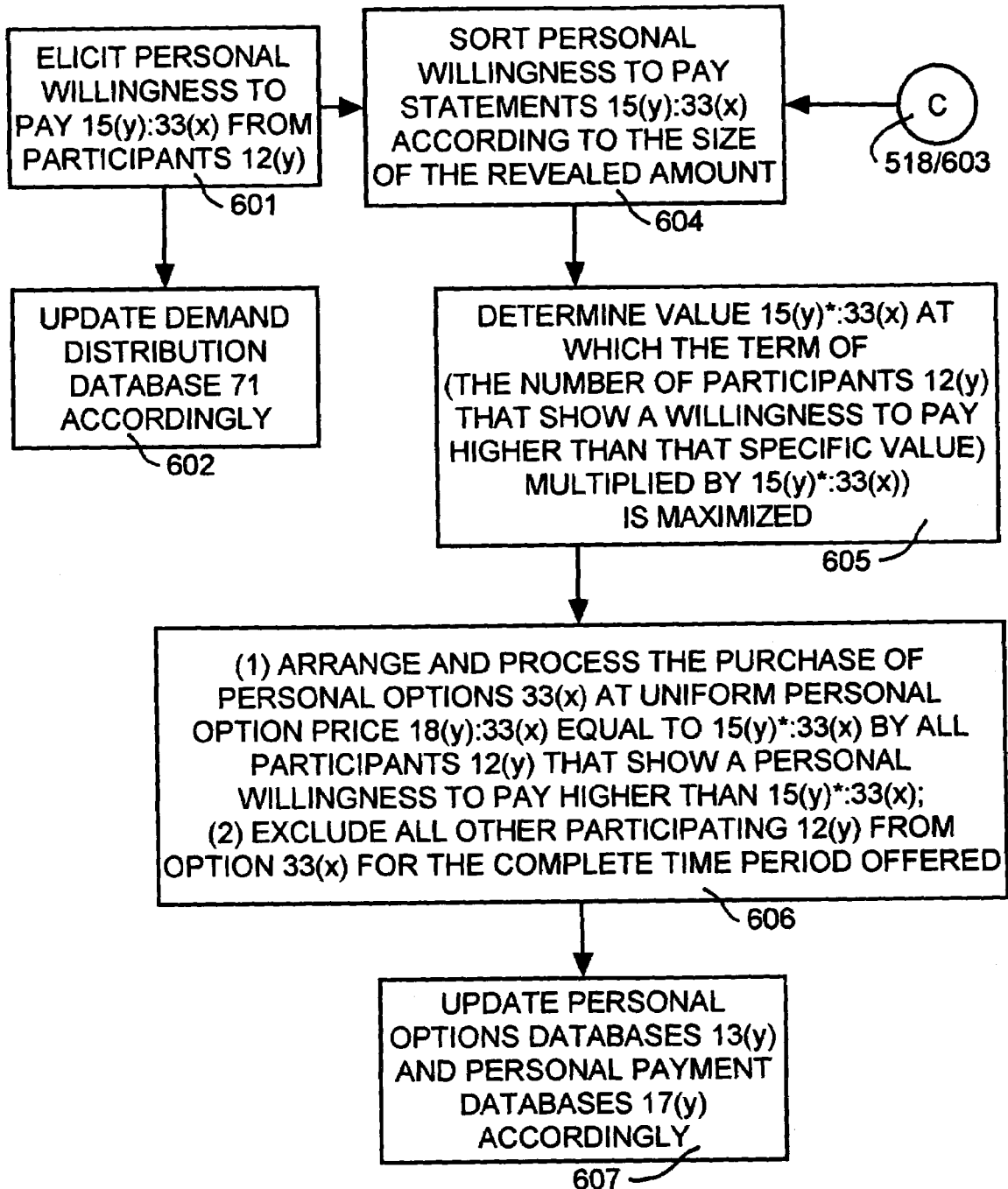
Fig.6: Option Auction
