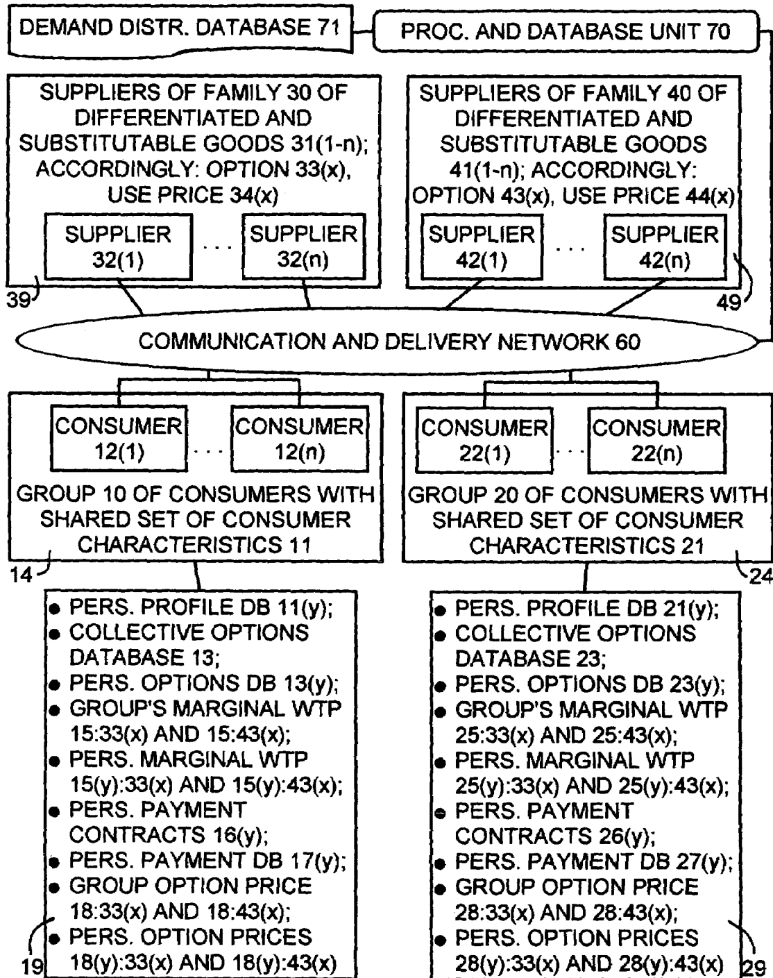
Fig.2: Overall Environment 80
