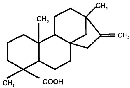
Isosteviol
