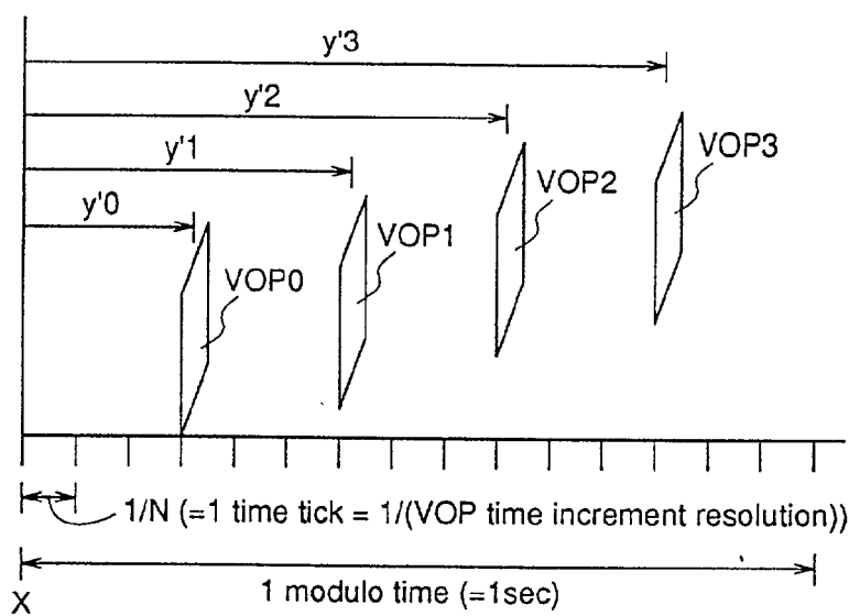
Fig.17 (b) frame cycle ( 1 fixed VOP increment = \text{VOP rate increment} \times \text{time tick} = M \times \frac{1}{N} )
