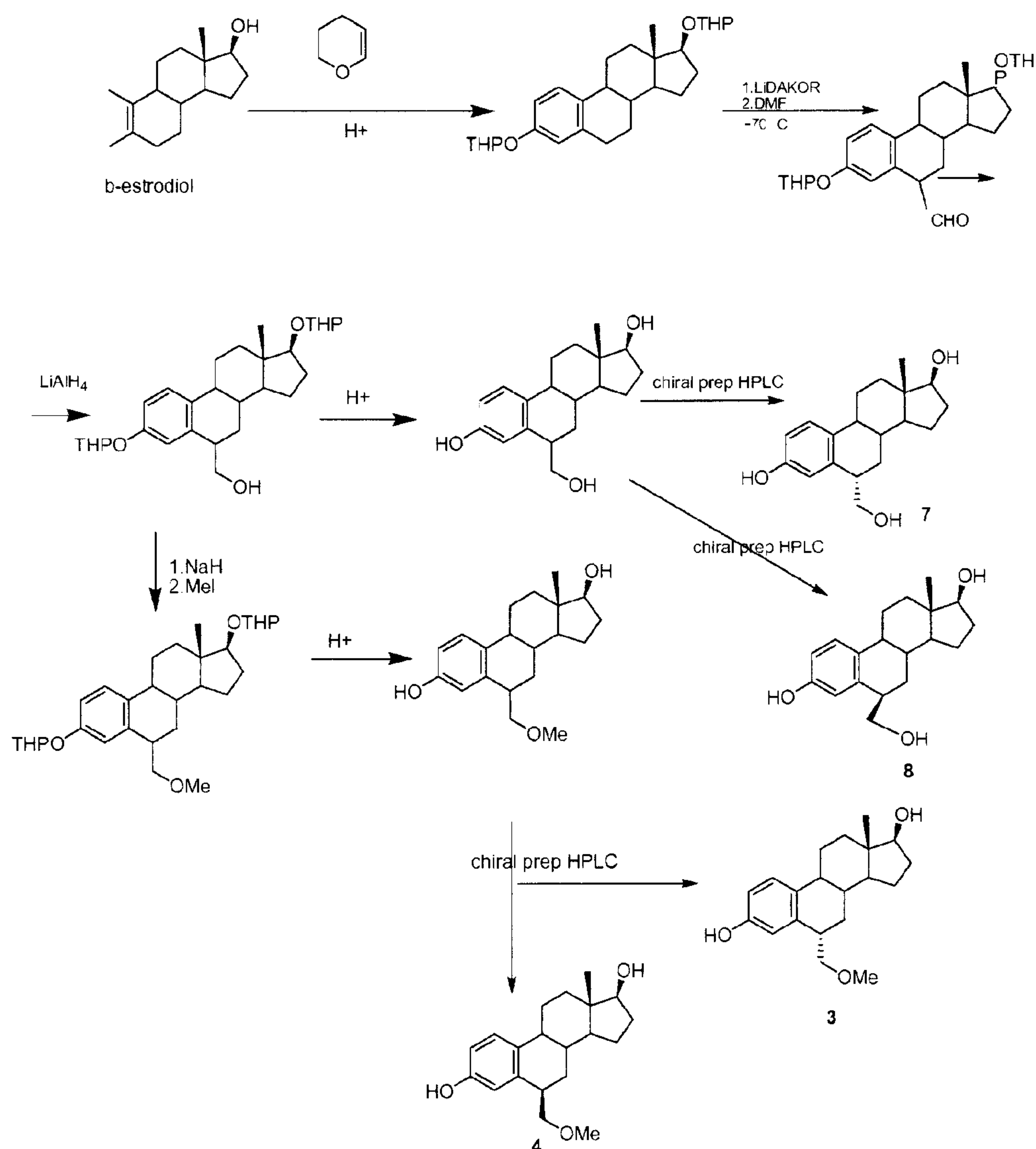
Scheme 2
