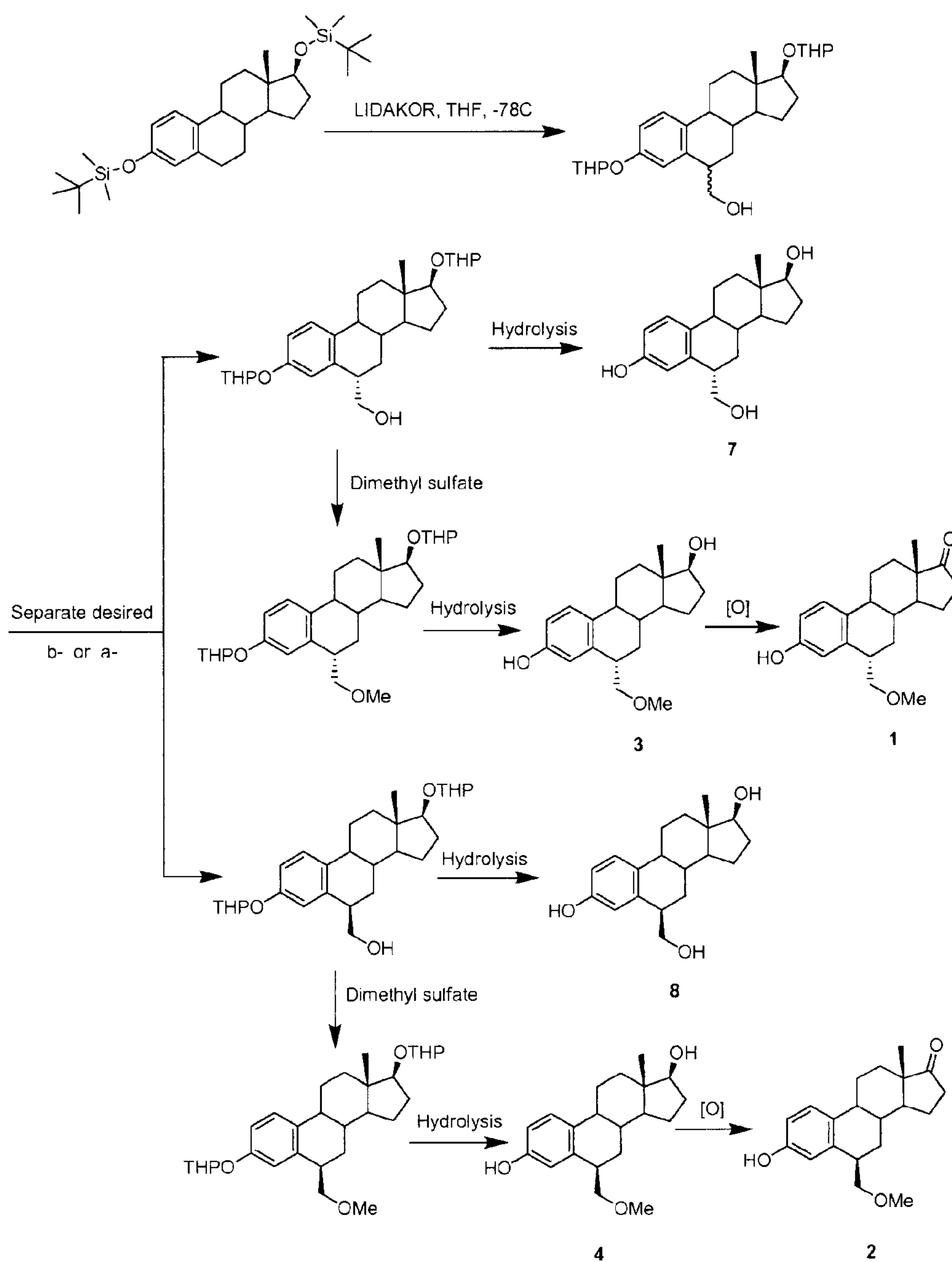
Scheme 1
