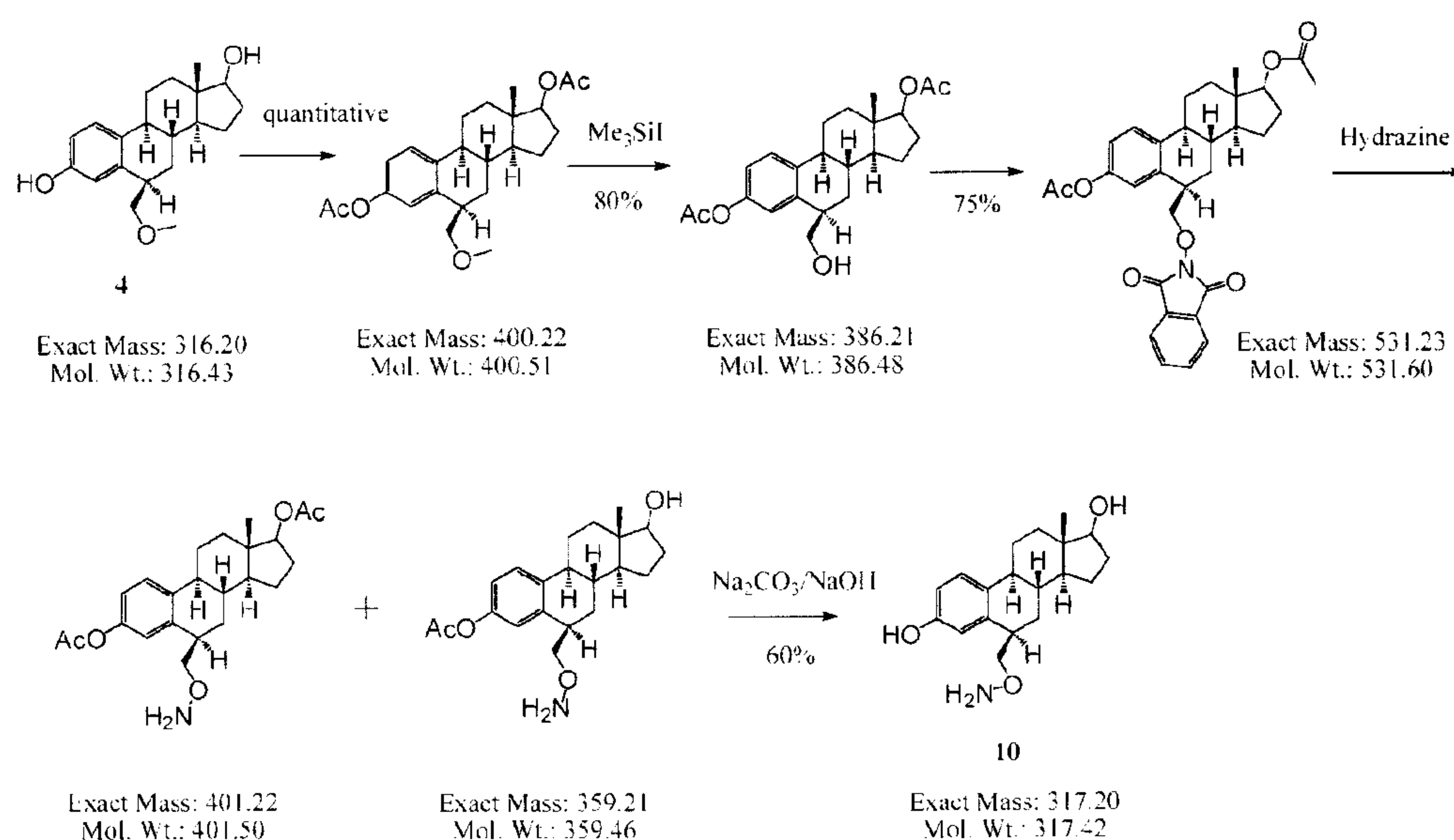
Scheme 3
