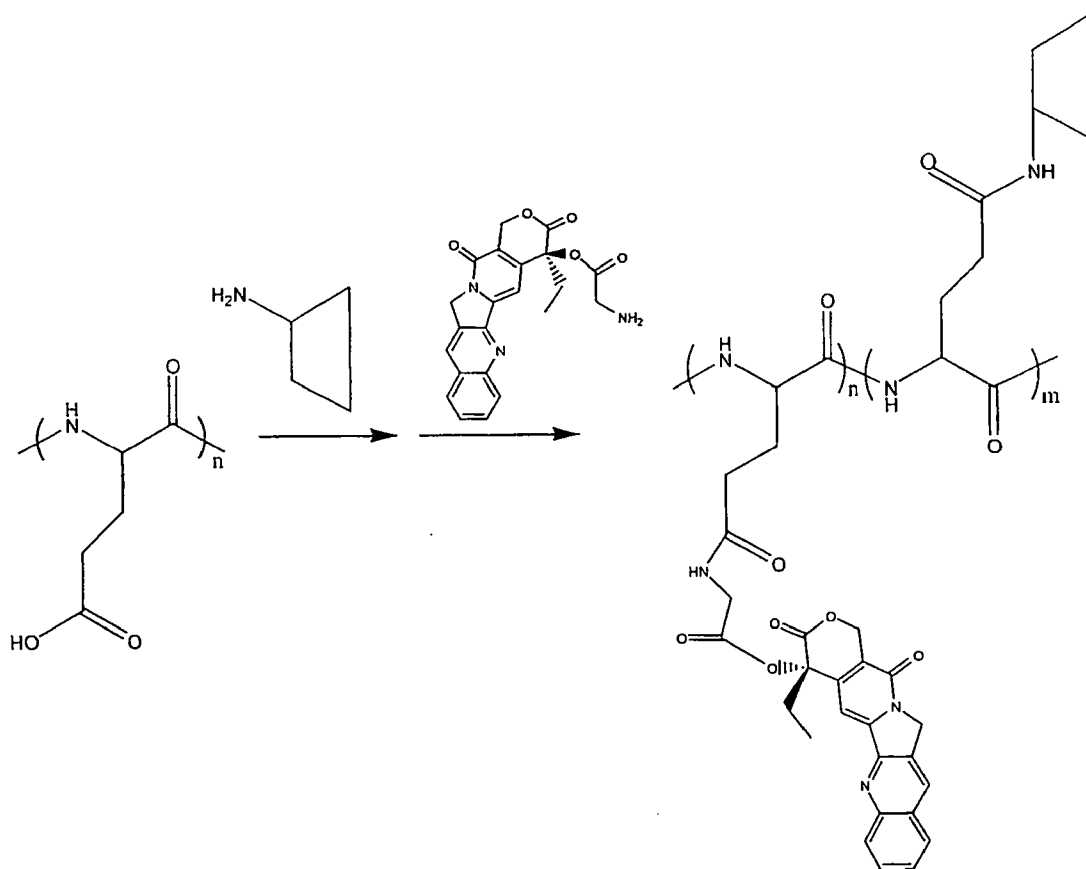
Scheme XII
