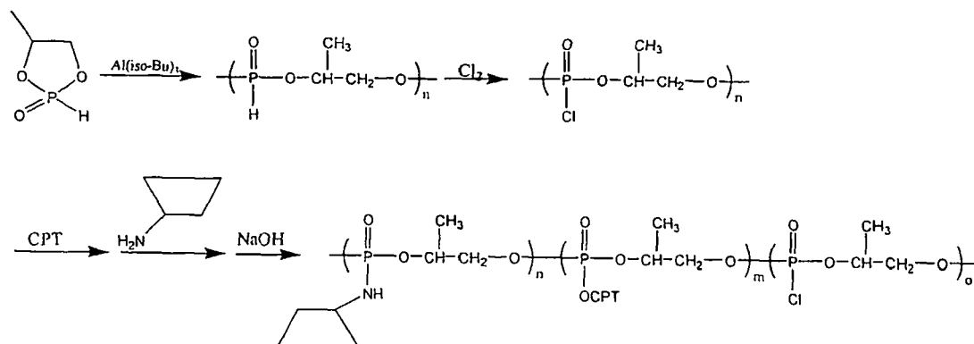
Scheme IX
