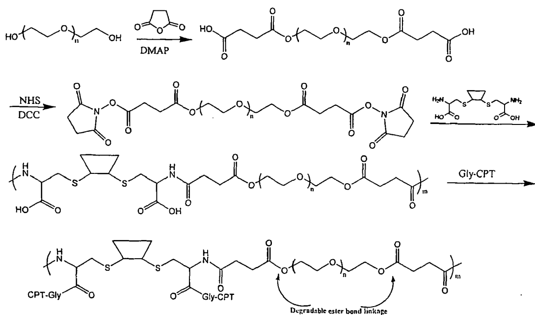
5 Scheme XIV
