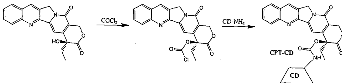
Scheme I
