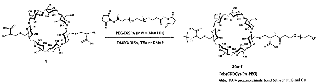
Scheme XXXVIIIa
