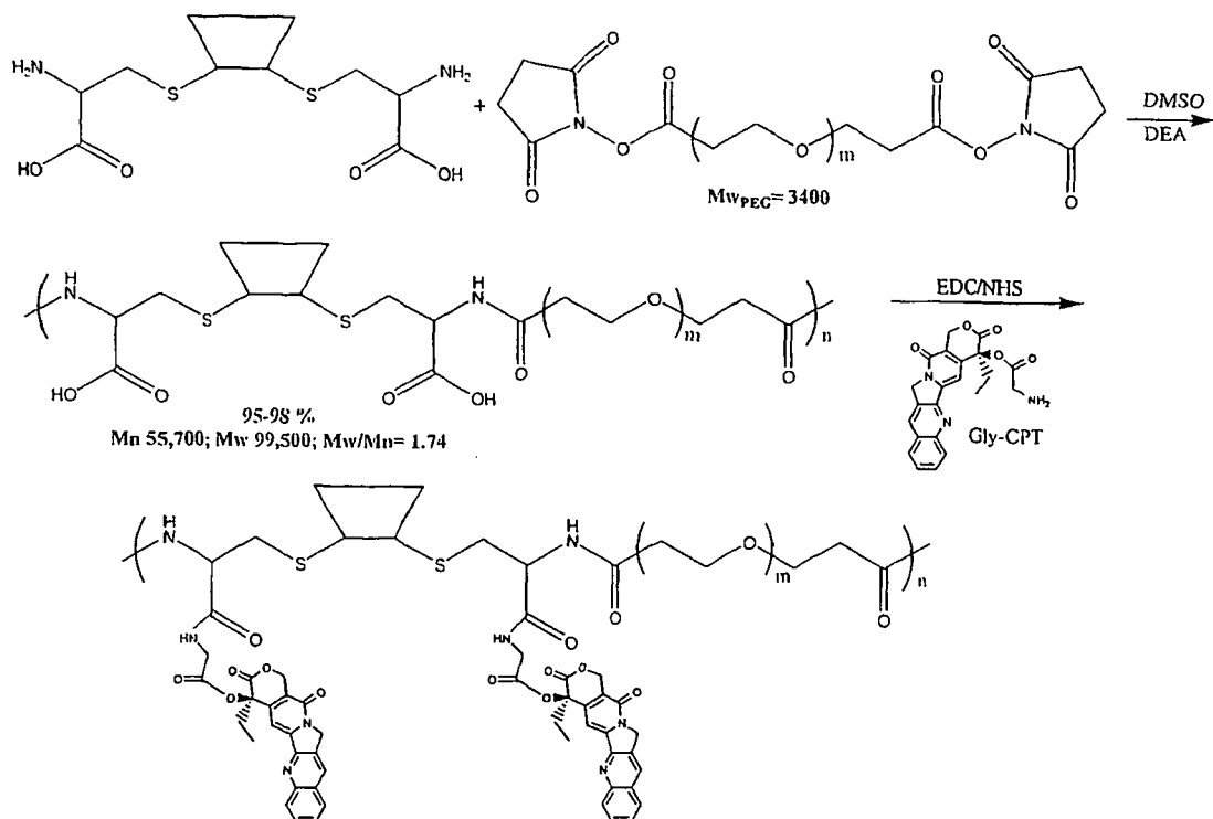
Scheme XIII
