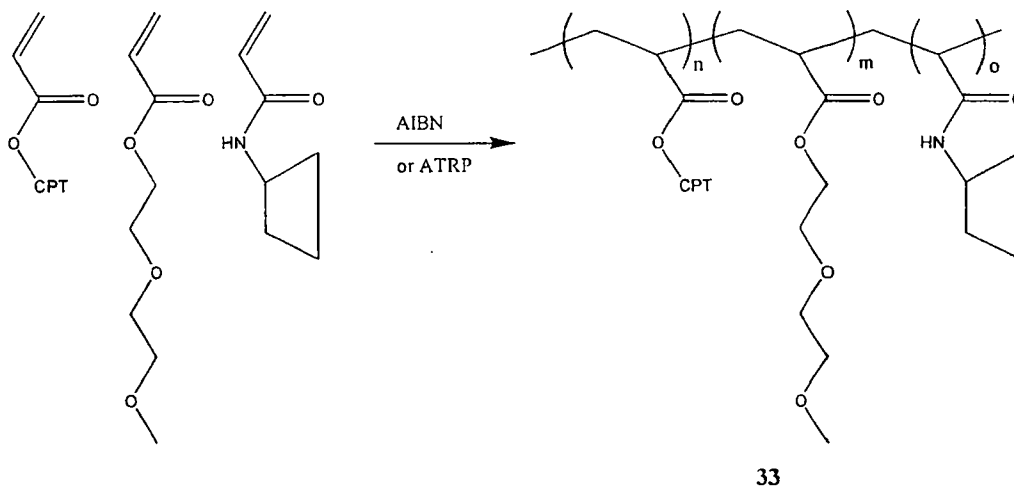
Scheme XXXV
