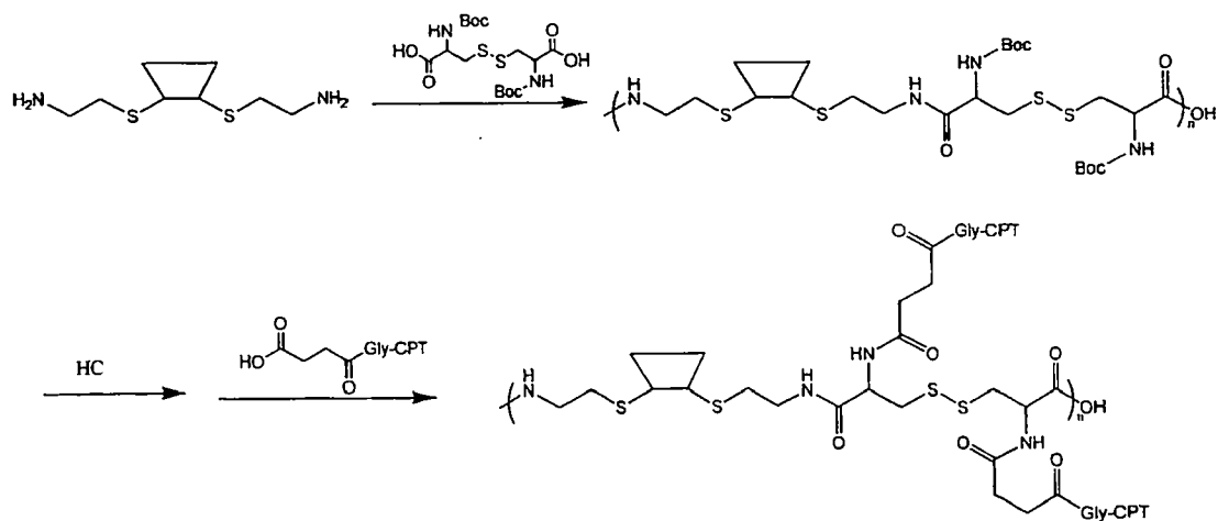
Scheme VII
