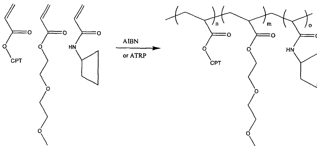
Scheme X
