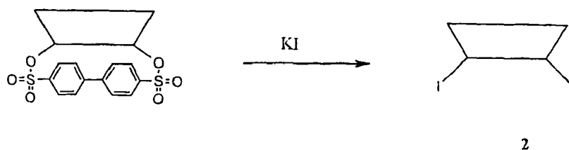
Scheme XVI
