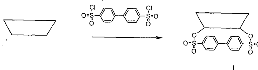
Scheme XV
