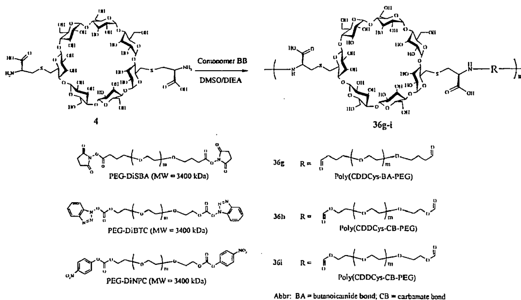
Scheme XXXVIIIb
