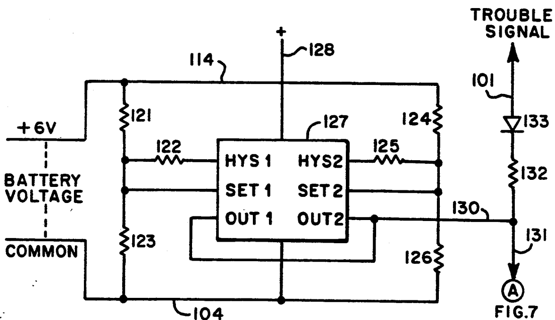
Low Voltage and High Voltage Supervisory Circuit 100
