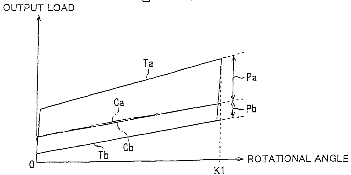
TORSION COIL SPRING + BUSHING
