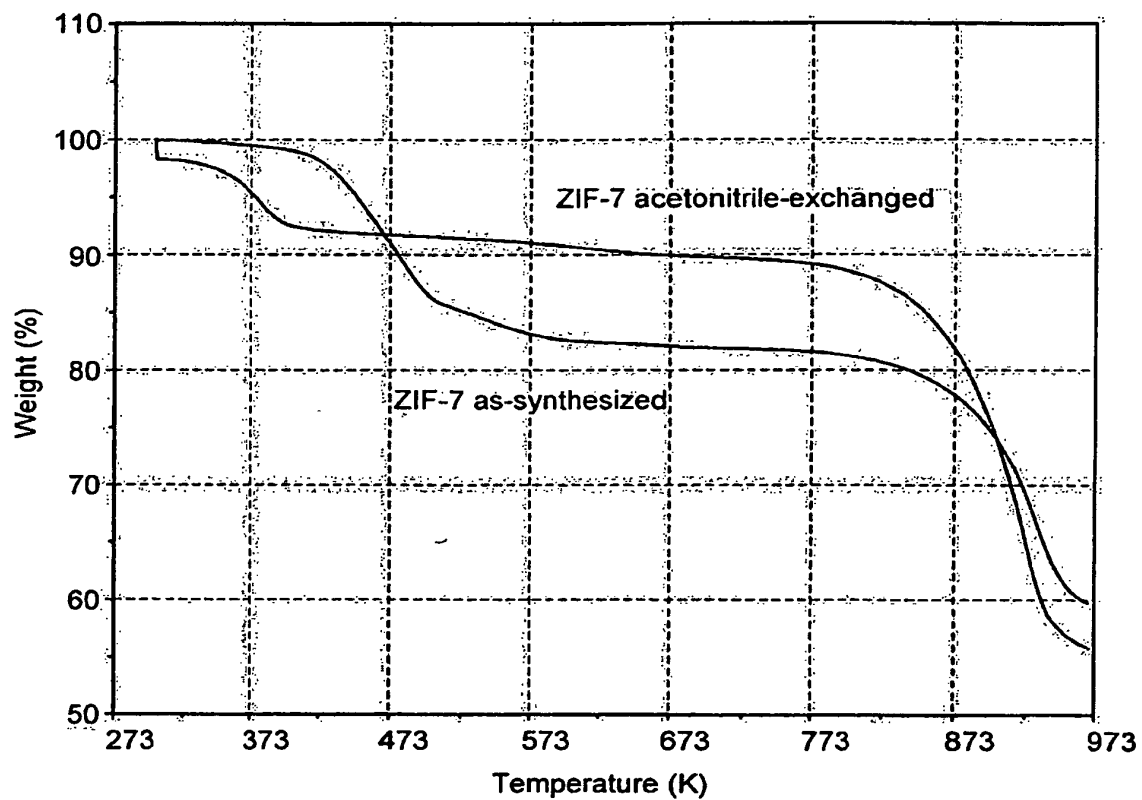
Thermogravimetric Analyses of ZIF-7
