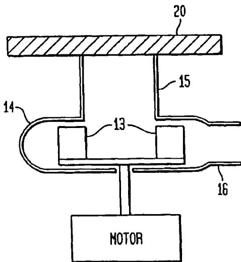
FIG. 14A (PRIOR ART)
