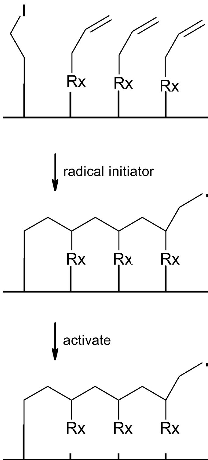
Figure 18, example 1. Radical polymerization
