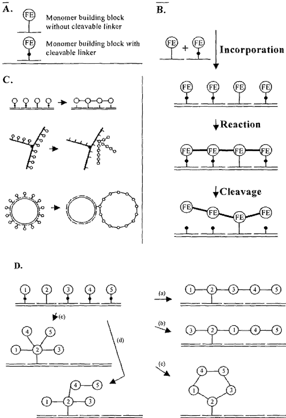
Figure 26. Chemical Display – principle.
