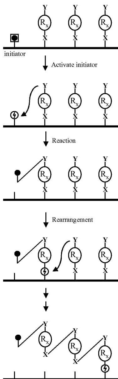
Figure 20. Zipping-polymerization and activation by rearrangement.
