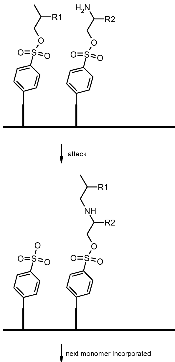
Figure 14, example 2. Polyamine formation and activation
