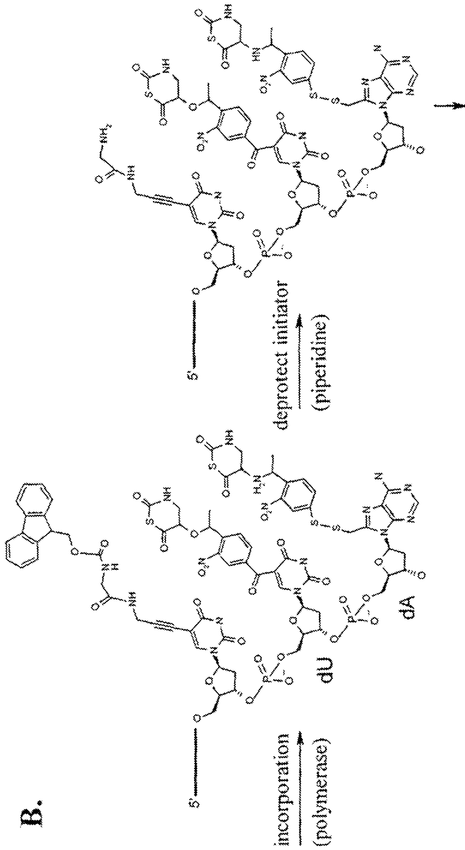
Figure 7. C-terminal tagging of a \beta -peptide – incorporation, polymerization, and activation. An example
