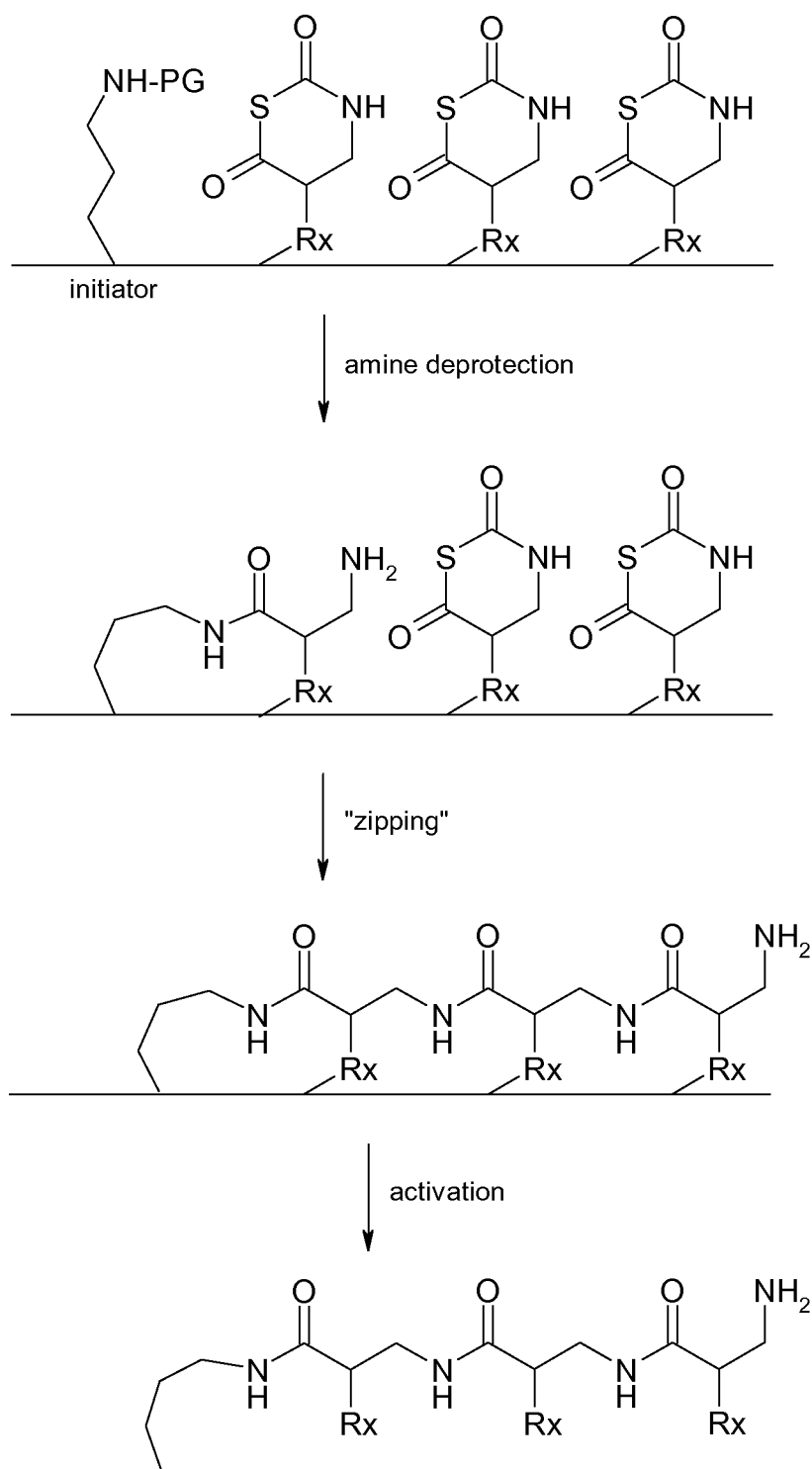
Figure 19, example 1. "Zipping" polymerization of N-thiocarboxyanhydrides, to form \beta -peptides
