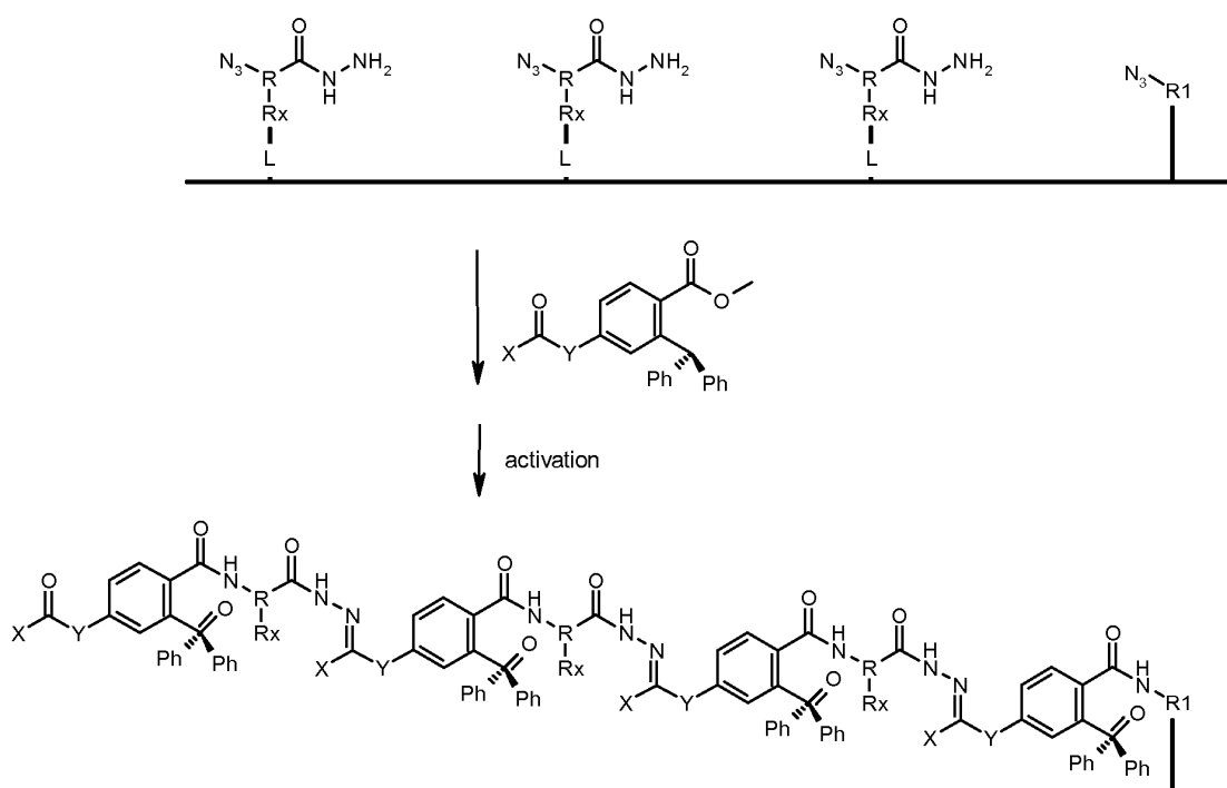
Figure 17, example 1. Fill-in polymerization by ketone-hydrazone reaction and by modified Staudinger ligation
