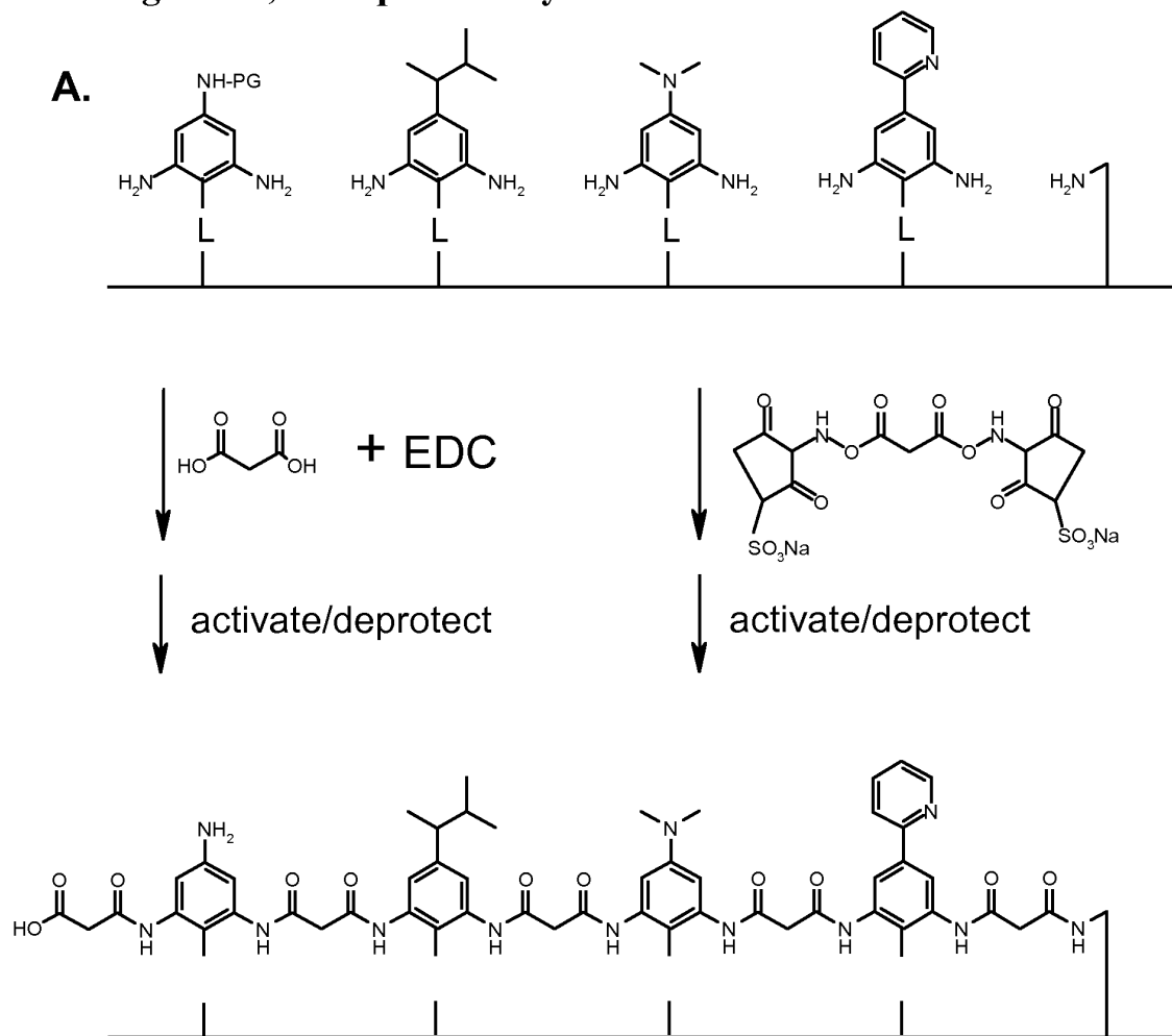
Figure 15, example 2. Polyamide formation.
