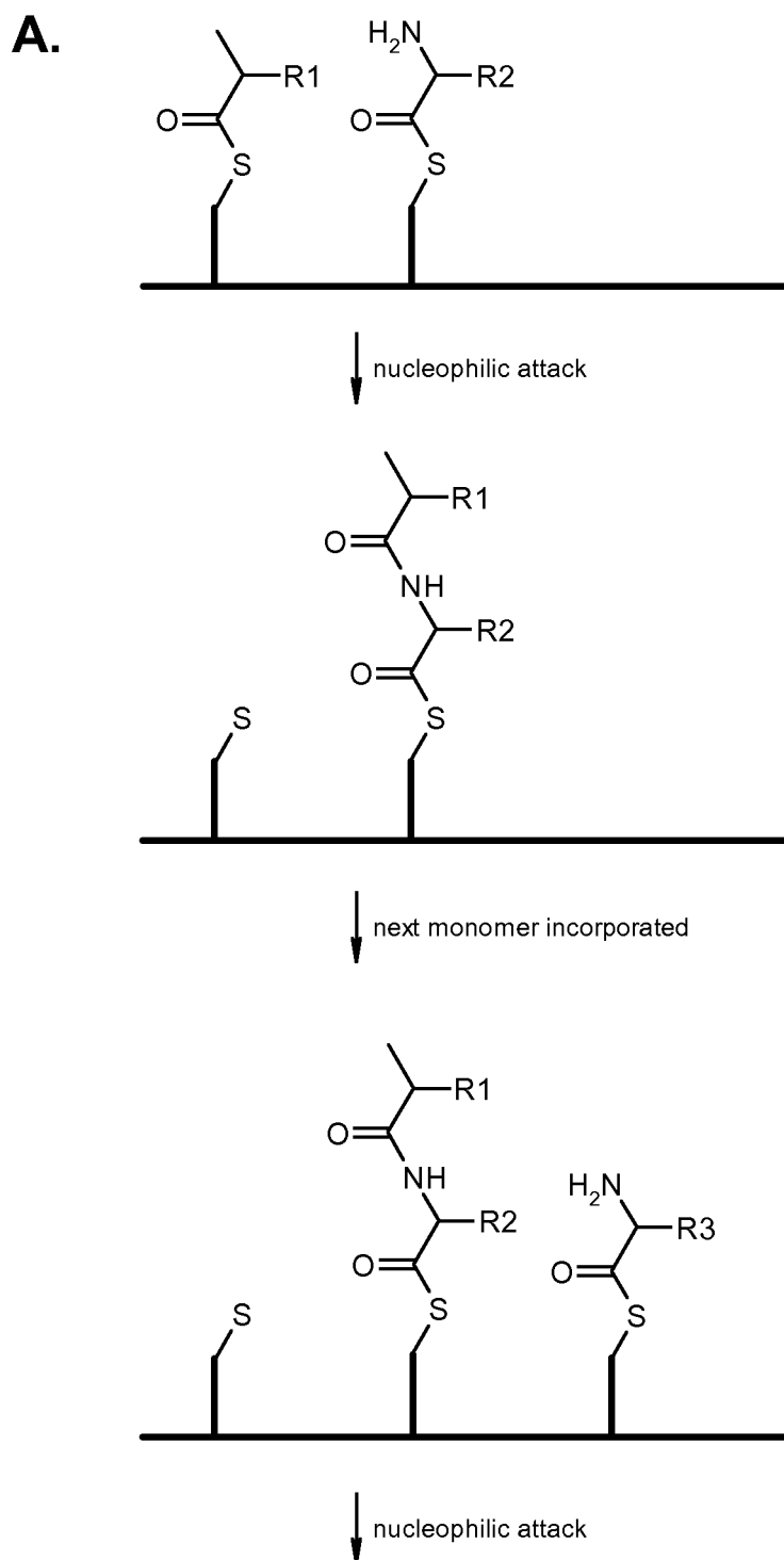
Figure 14, example 1. Polymerization and activation (thioesters)
