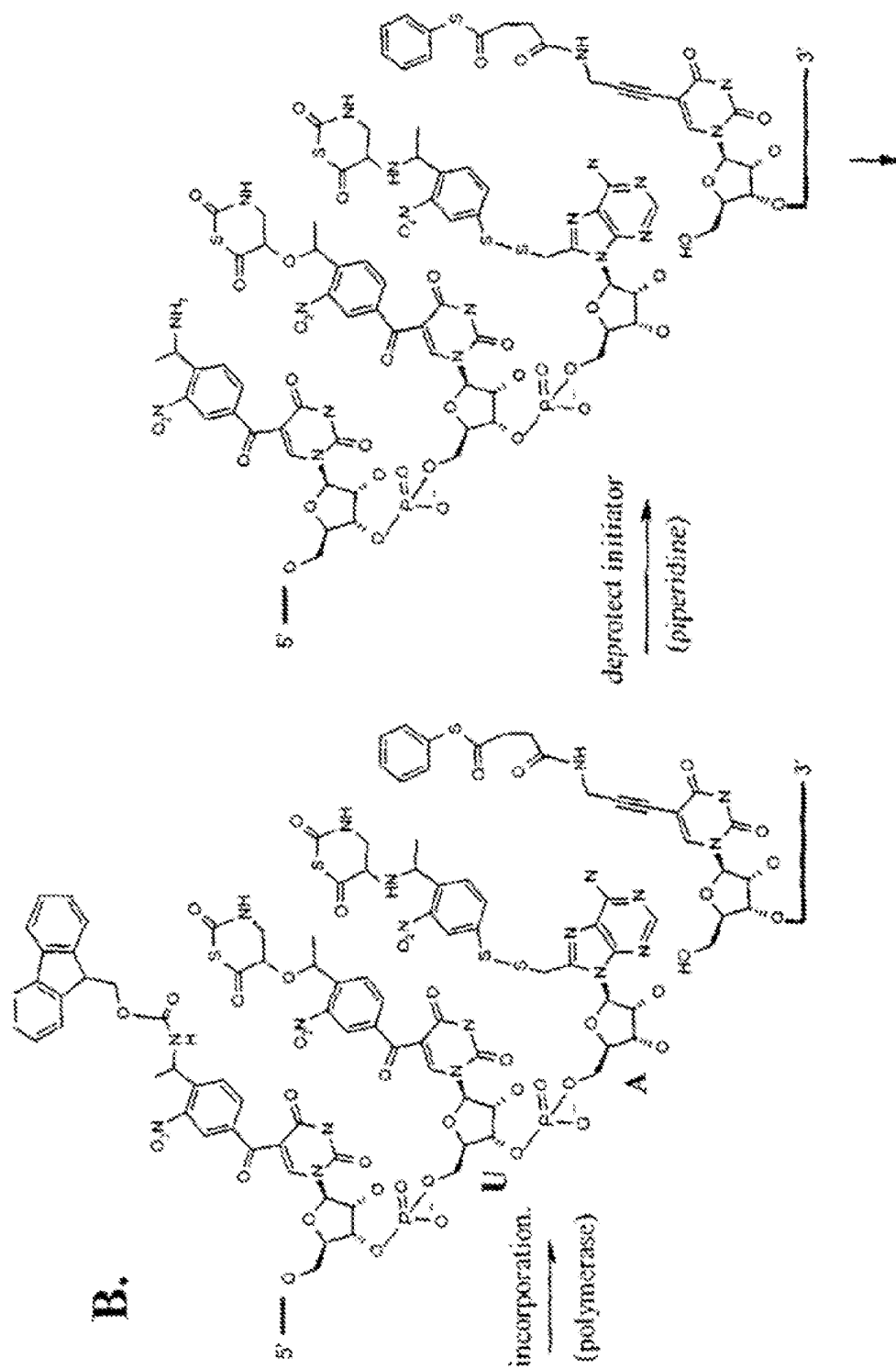
Figure 8. N-terminal tagging of a \beta -dipeptide - incorporation, polymerization and activation.
