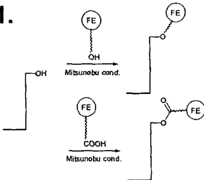
Figure 36. Formation of Monomer Building Blocks - Examples
