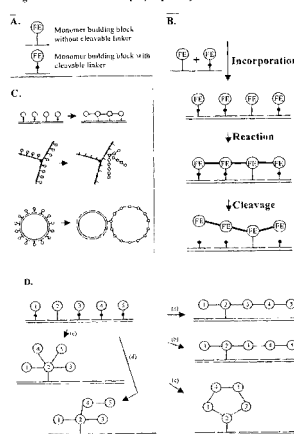
Figure 26. Chemical Display – principle.
