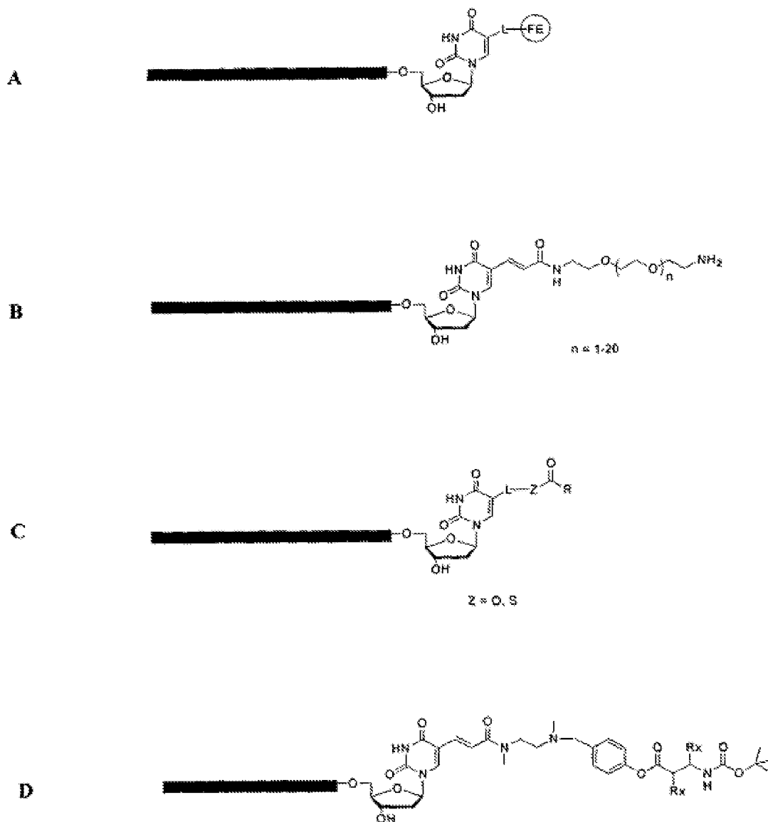
Figure 37. A derivatized oligonucleotide as building block.
