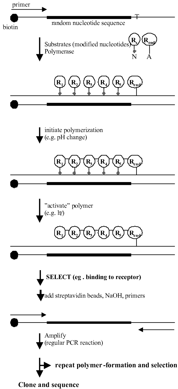
Figure 1. Chemical Display – Principle.
