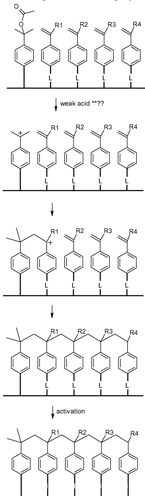
Figure 18, example 2. Cationic polymerization
