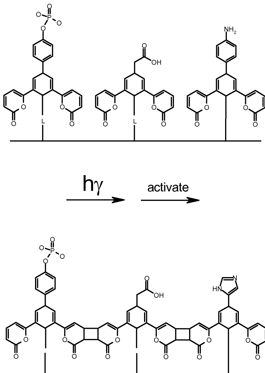
Figure 11, ex.1. Coumarin-based polymerization.
