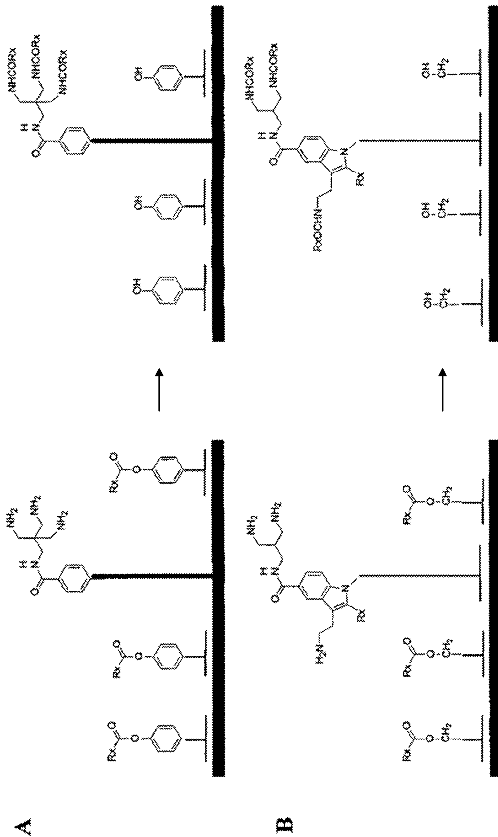
Figure 43. Templated synthesis of organic compounds - examples
