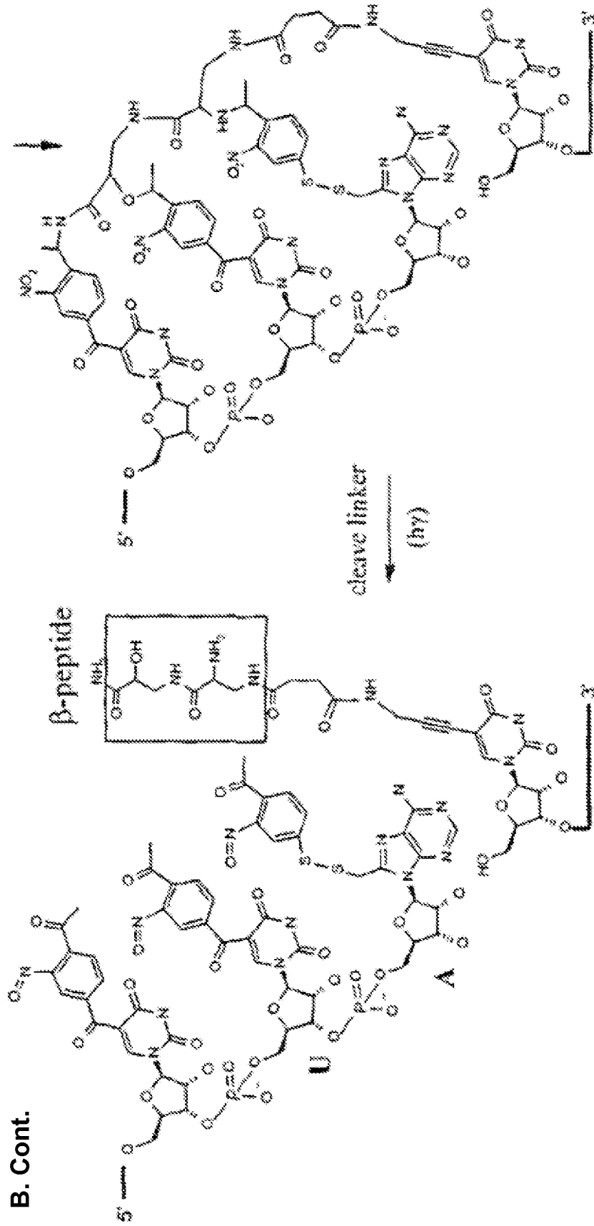
Figure 8. N-terminal tagging of a \beta -dipeptide - incorporation, polymerization and activation.
