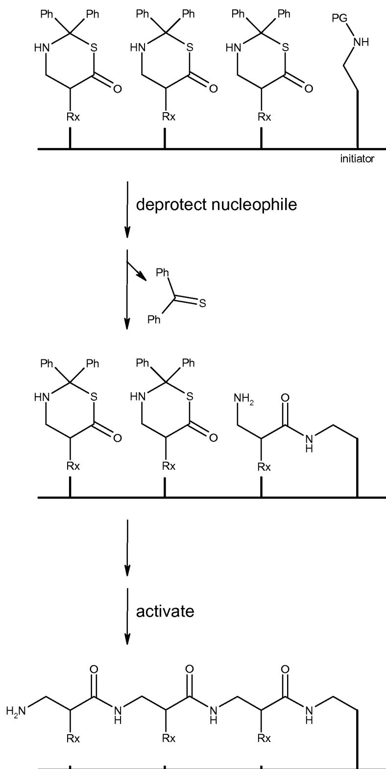
Figure 19, example 2. "Zipping" polymerization of 2,2-diphenylthiazinane units to form \beta -peptides.
