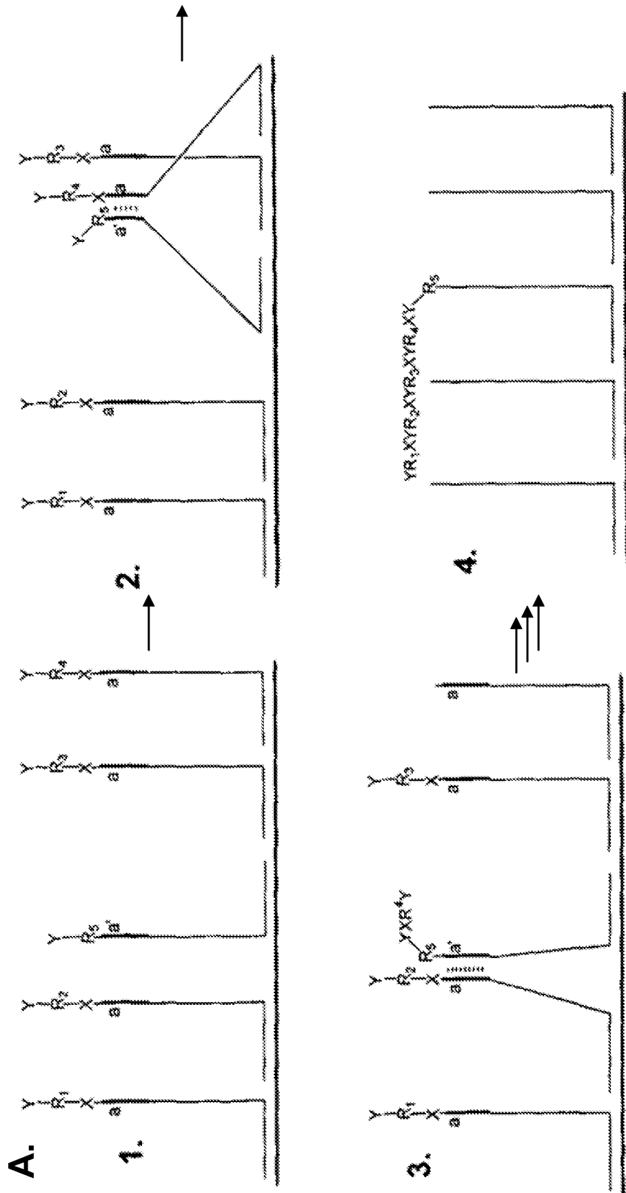
Figure 42. Use of Zipper Box
