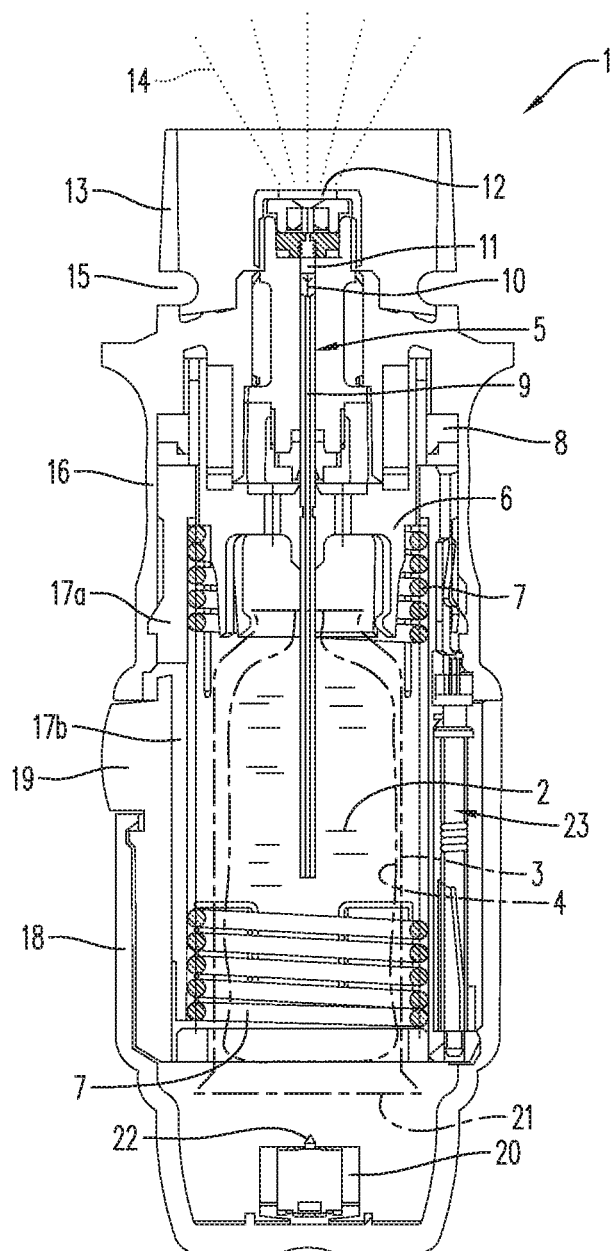
FIG. 1 (PRIOR ART)
