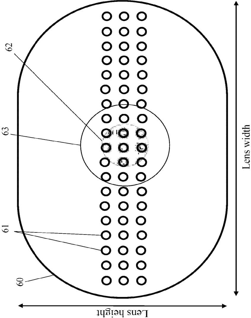
Refractive optical elements (ROE) embedded into a spectacle lens
