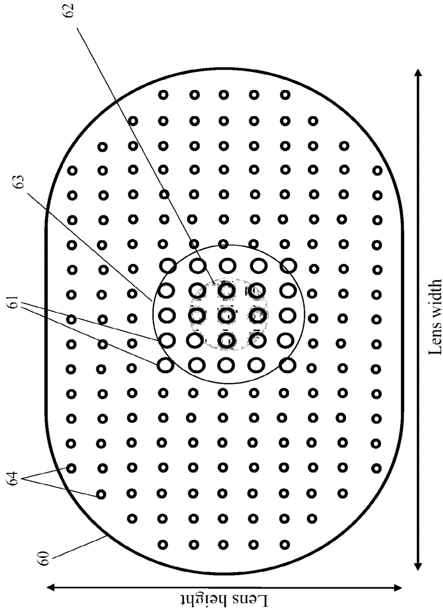
Refractive optical elements (ROE) embedded into a spectacle lens FIGURE 15B
