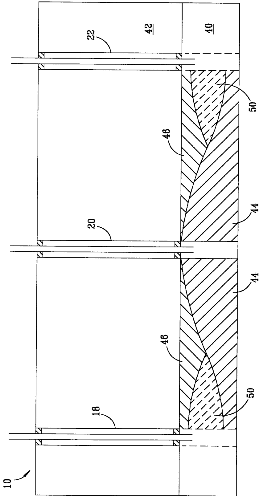
FIG. 3 (PRIOR ART)
