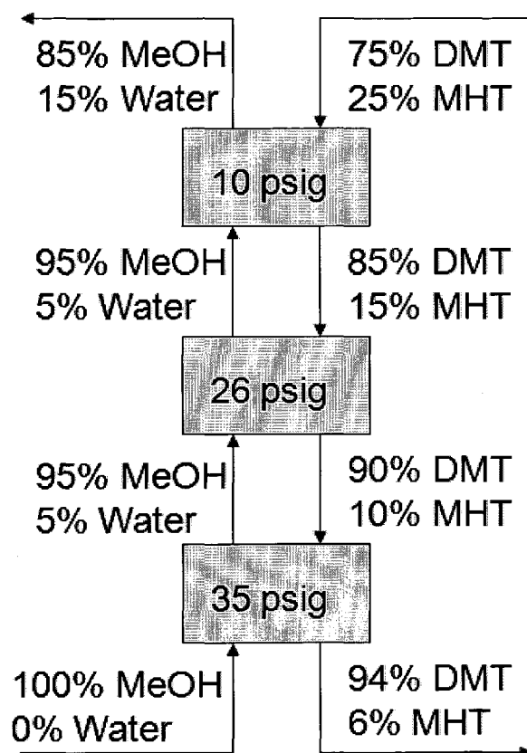
Figure 2. MHT Reactor: Three Stage Model
