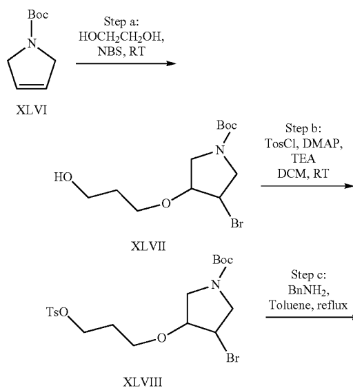
Scheme 7:
