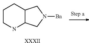
Scheme 4:
