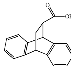
Intermediate product 2
