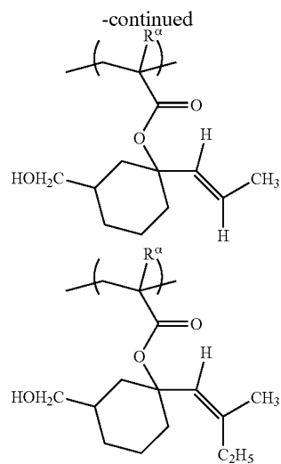
[Chemical Formula 19.]
