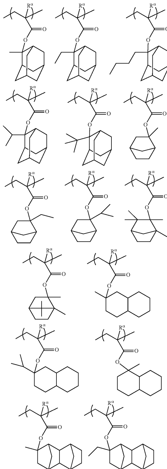
[Chemical Formula 16.]
