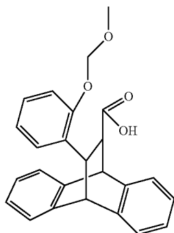
Intermediate product 10
