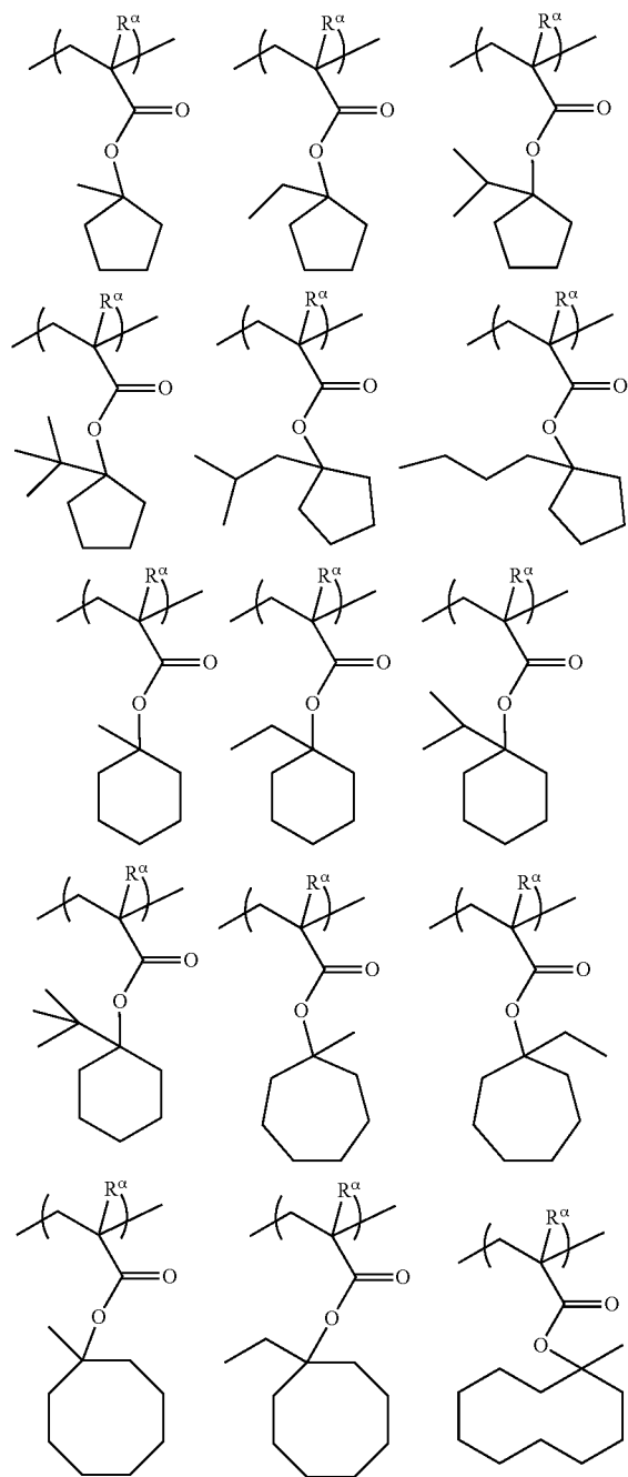
[Chemical Formula 17.]
