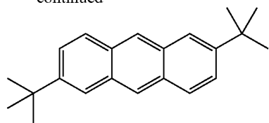
Intermediate product 15
