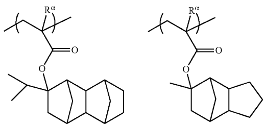
[Chemical Formula 17.]
