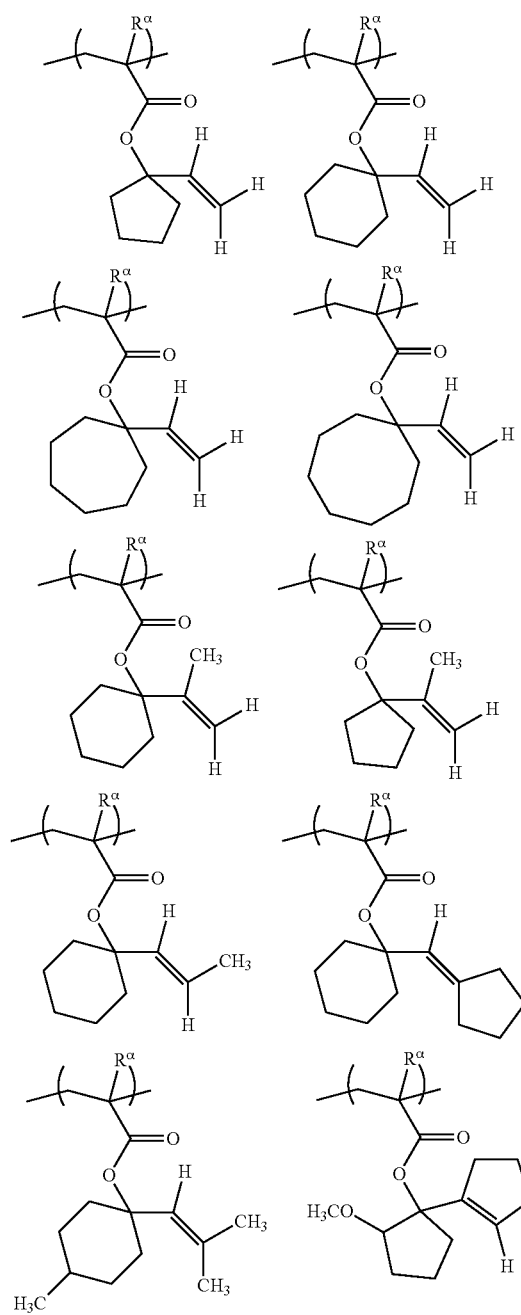
[Chemical Formula 18.]
