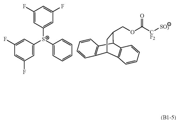
[Chemical Formula 66.]
