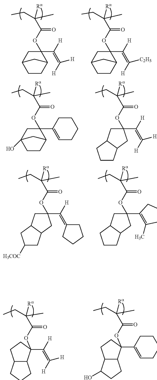
[Chemical Formula 20.]
