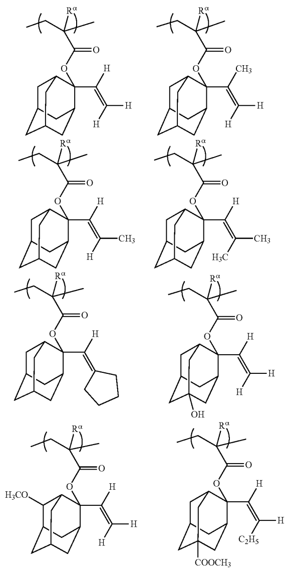
[Chemical Formula 19.]
