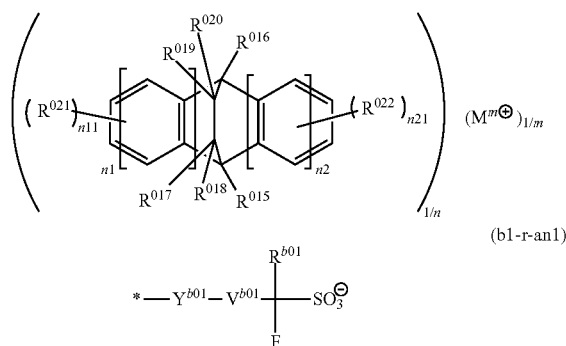
Chemical Formula 64.
