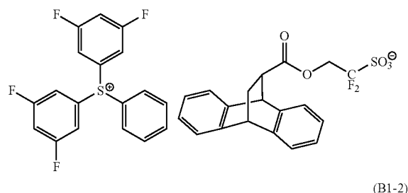
[Chemical Formula 65.]
