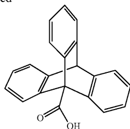
Intermediate product 12
