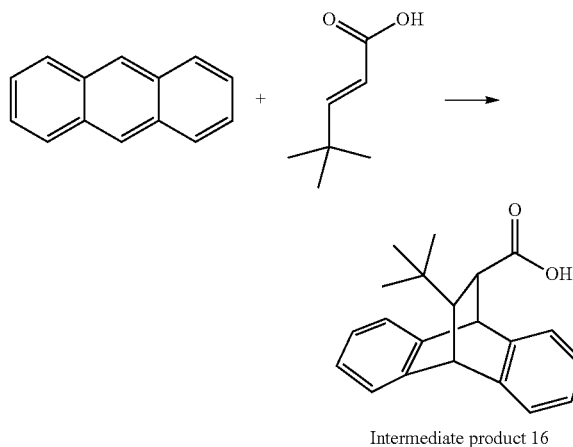
Intermediate product 16
